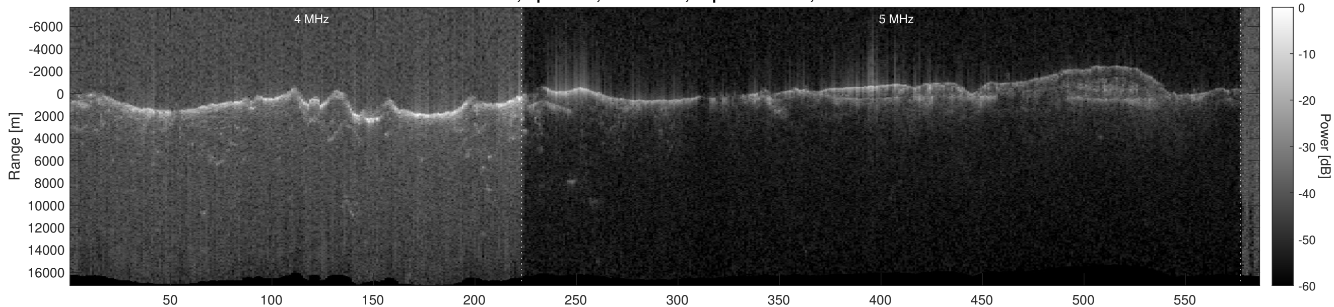
Orbit 21257, Optimized, No Window, Depth-Corrected, Channel 2
