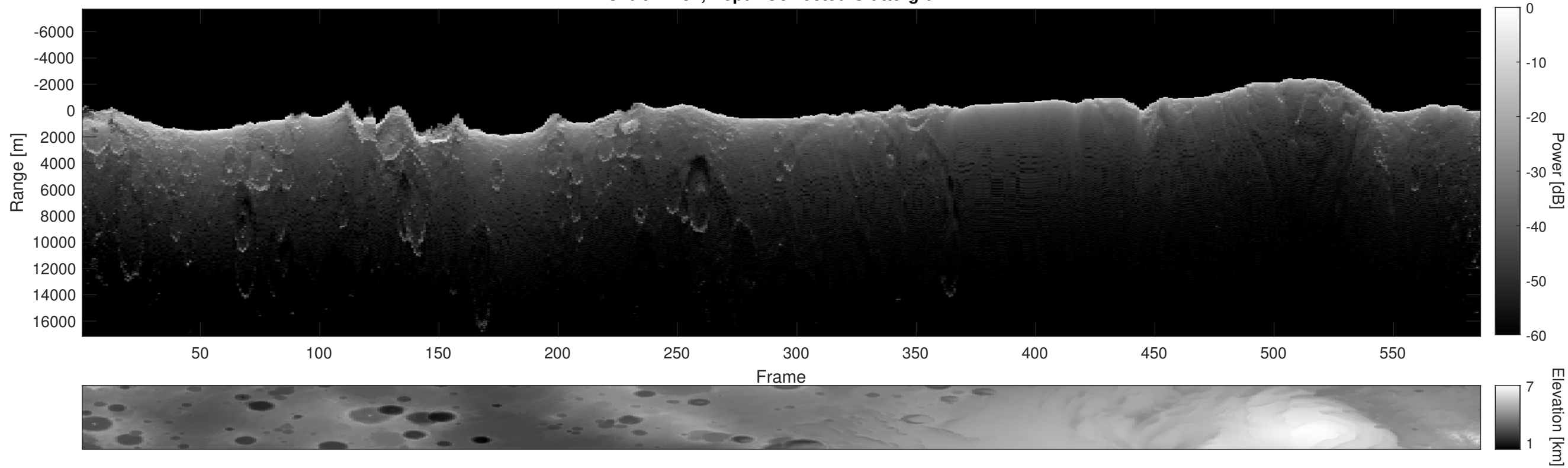
Orbit 21257, Depth-Corrected Cluttergram
