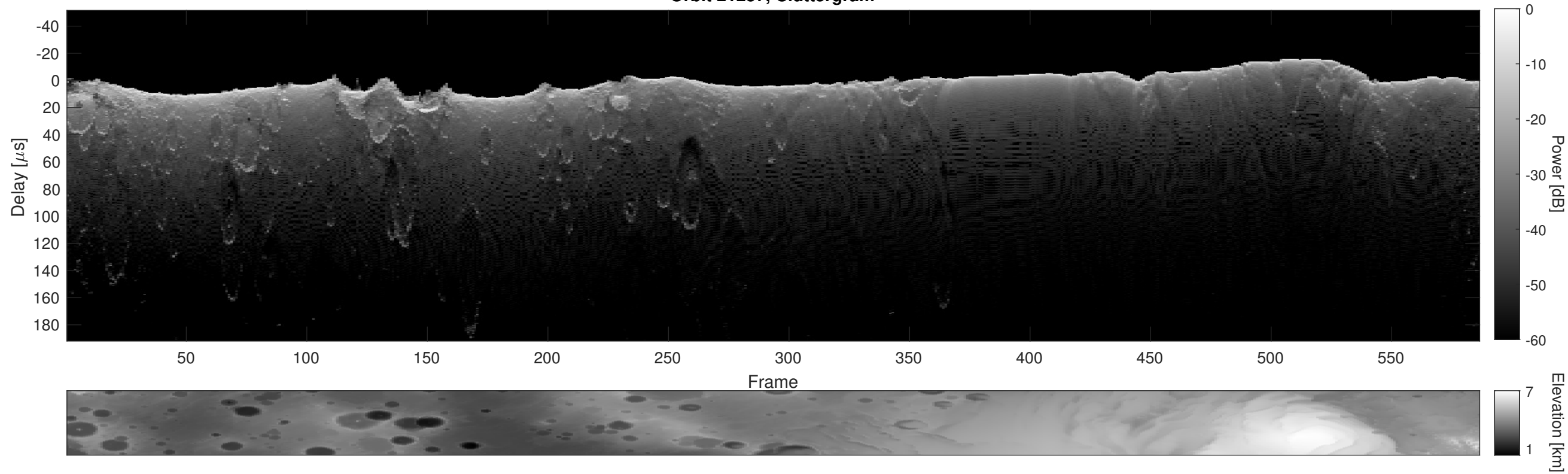
Orbit 21257, Cluttergram
