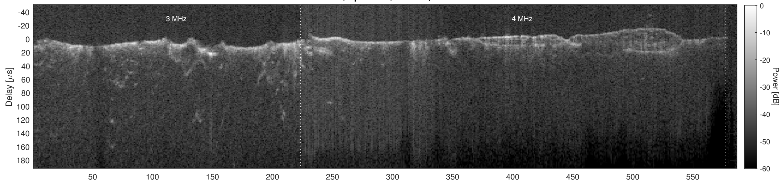
Orbit 21257, Cluttergram
