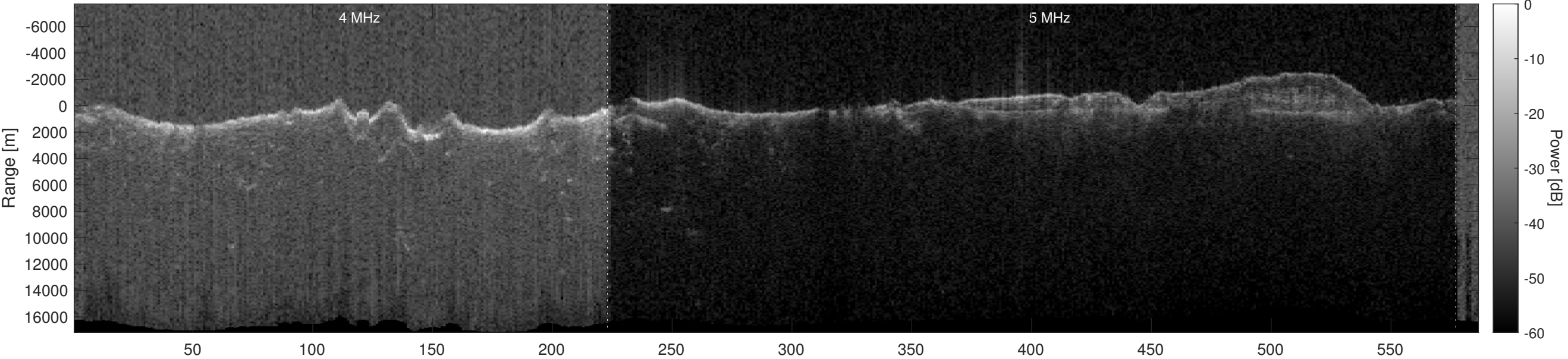
Orbit 21257, Optimized, Window, Depth-Corrected, Channel 2
