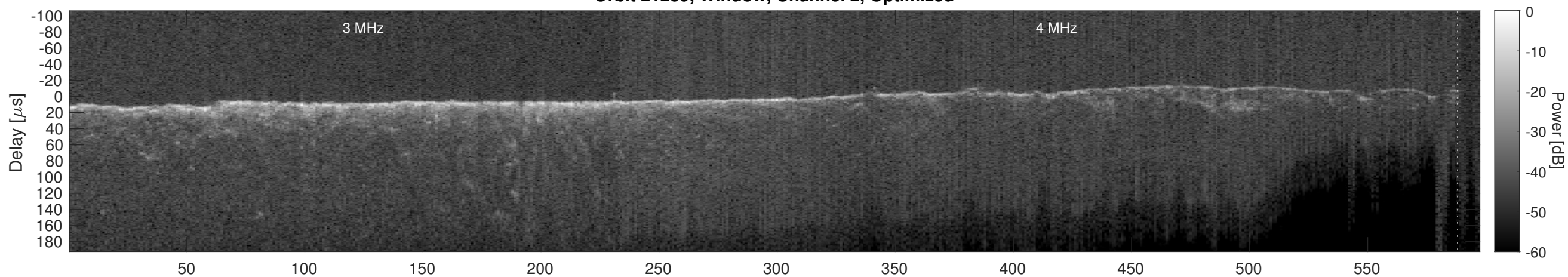
Orbit 21259, Cluttergram
