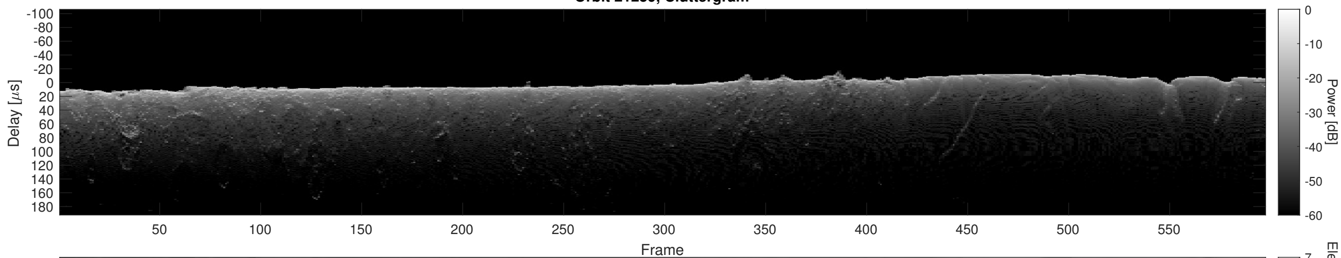
Orbit 21259, Cluttergram
