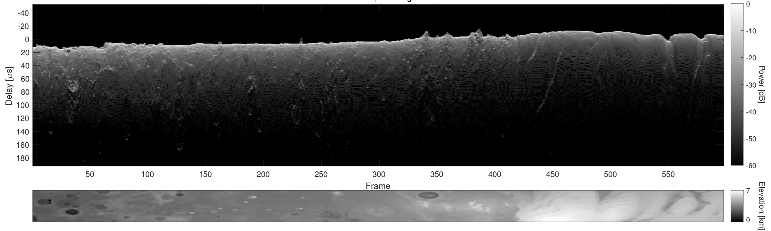
Orbit 21259, Cluttergram
