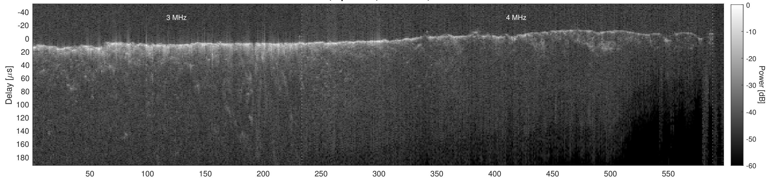
Orbit 21259, Cluttergram
