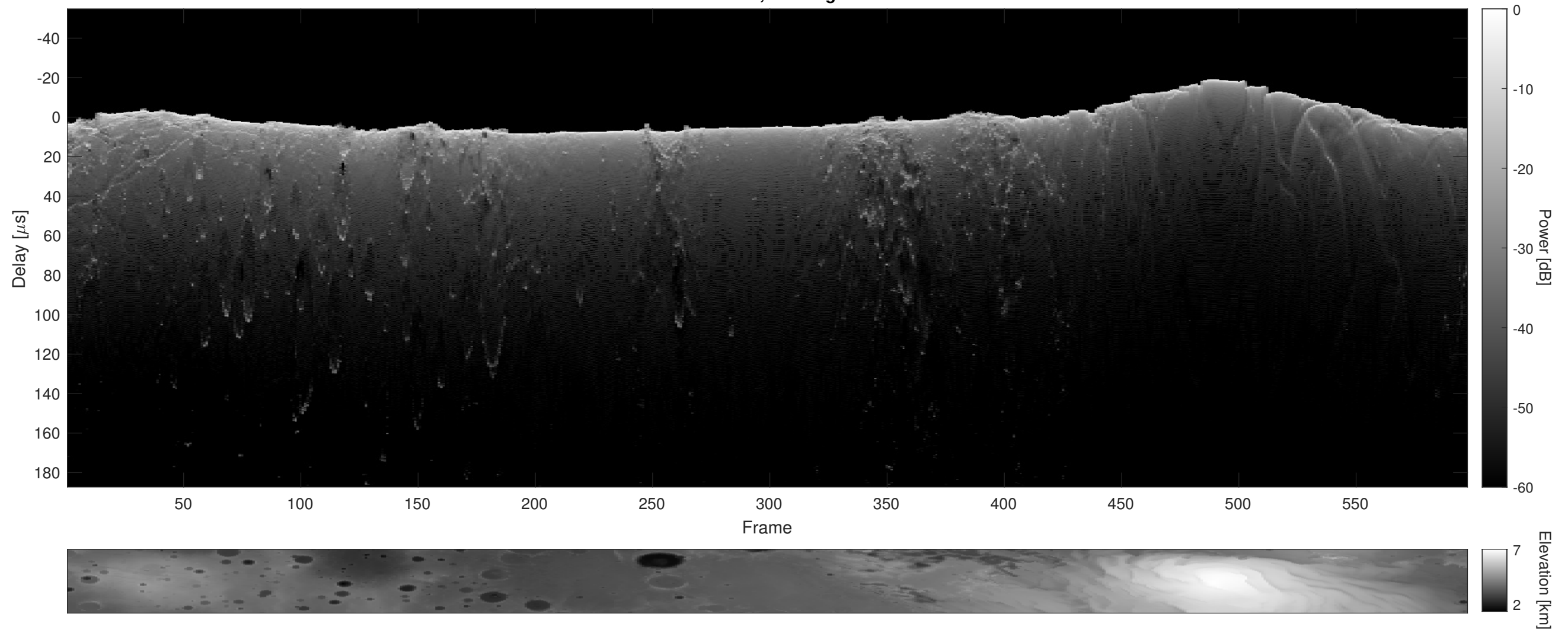
Orbit 21260, Cluttergram
