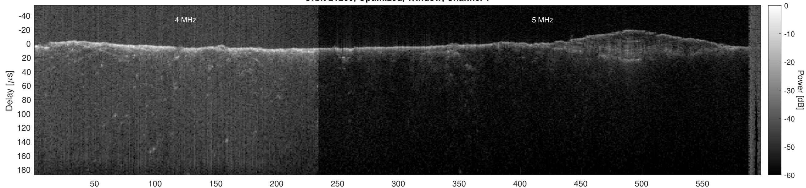
Orbit 21260, Optimized, Window, Channel 2
