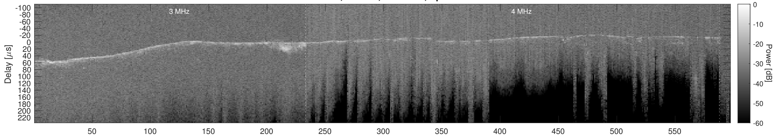
Orbit 21262, Cluttergram
