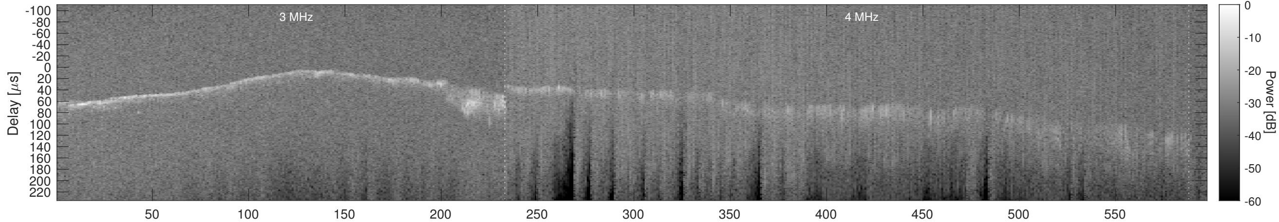
Orbit 21262, Window, Channel 2, Chapman
