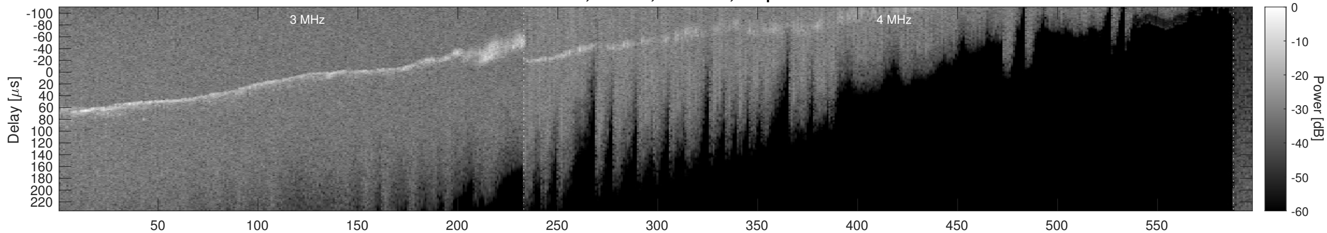
Orbit 21262, Window, Channel 2, Optimized
