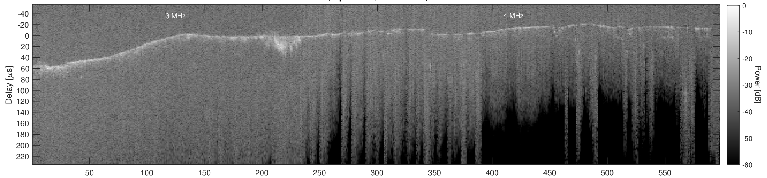
Orbit 21262, Cluttergram
