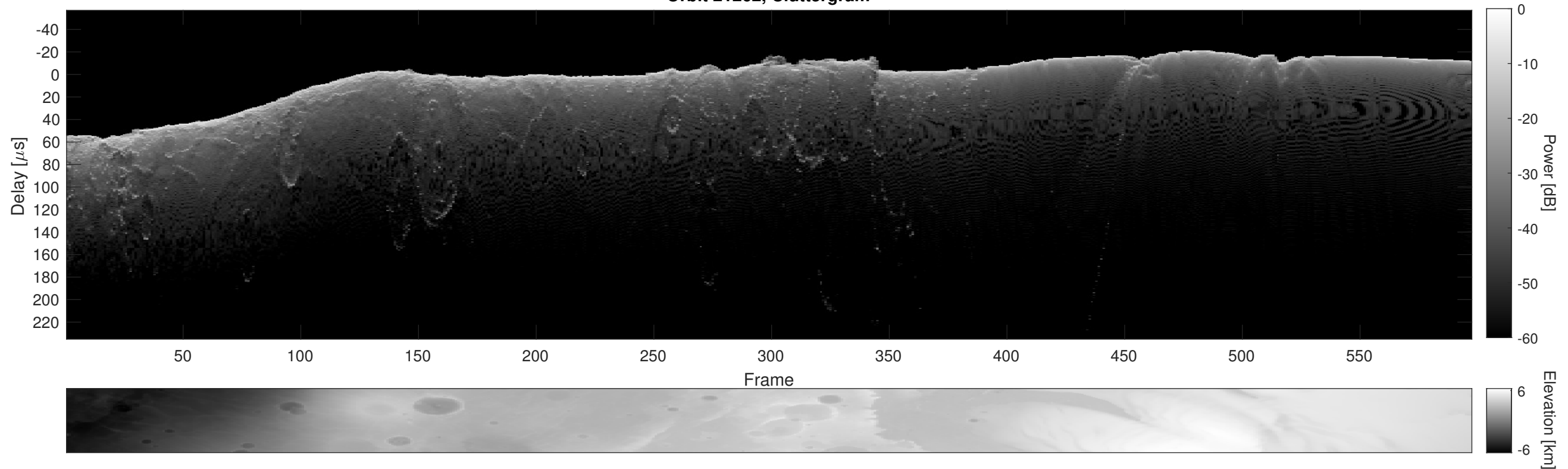
Orbit 21262, Cluttergram
