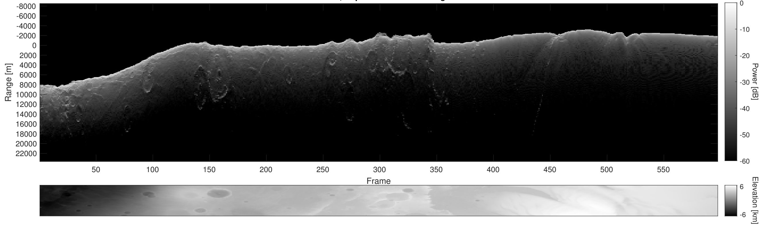
Orbit 21262, Depth-Corrected Cluttergram
