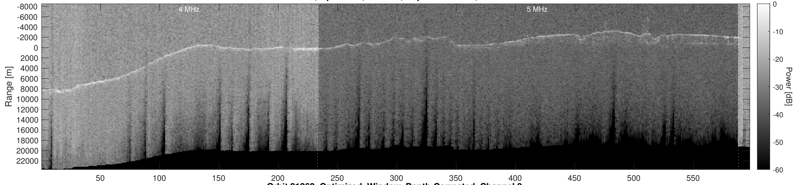
Orbit 21262, Optimized, Window, Depth-Corrected, Channel 2
