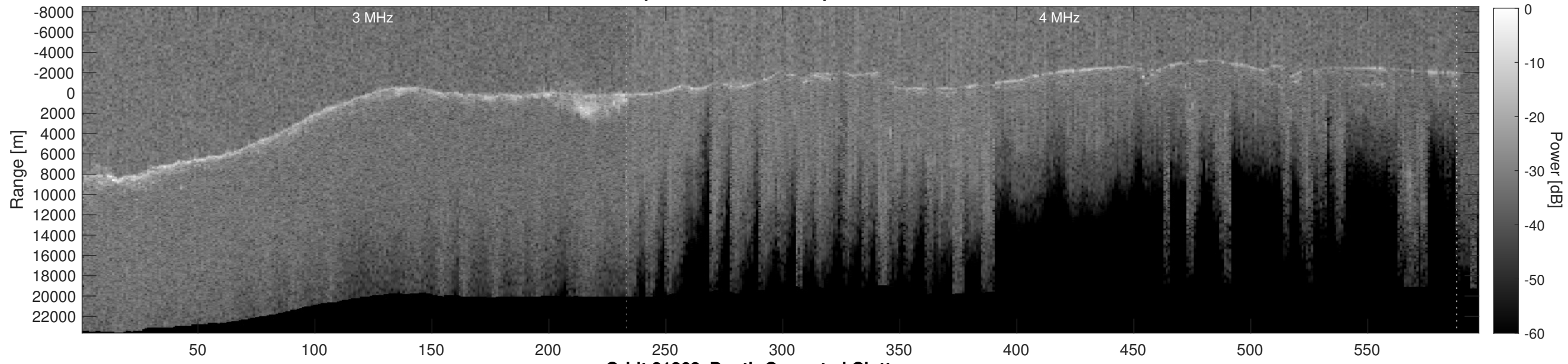
Orbit 21262, Depth-Corrected Cluttergram
