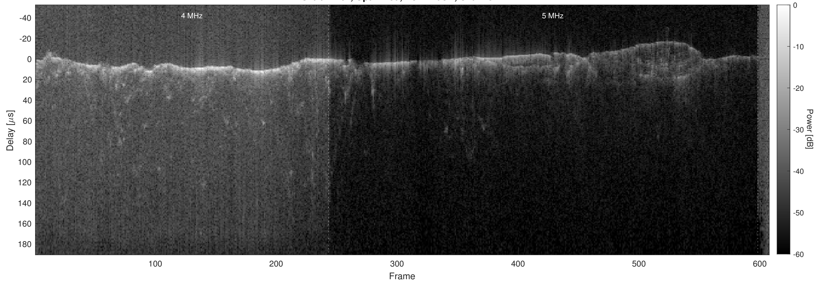
Orbit 21264, Optimized, No Window, Channel 2
