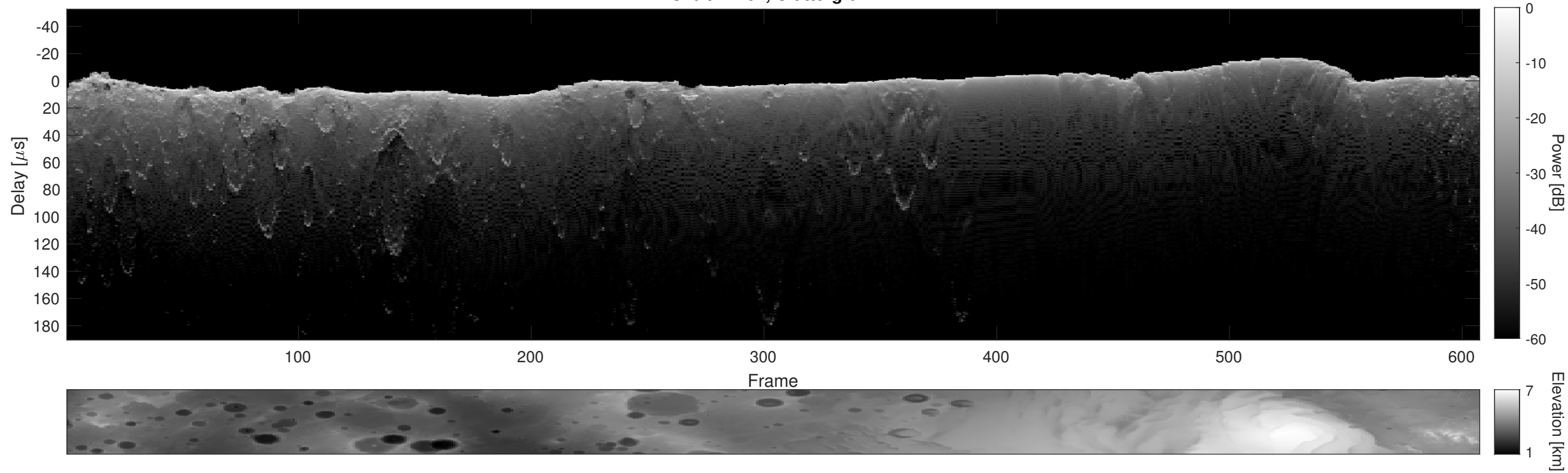
Orbit 21264, Cluttergram
