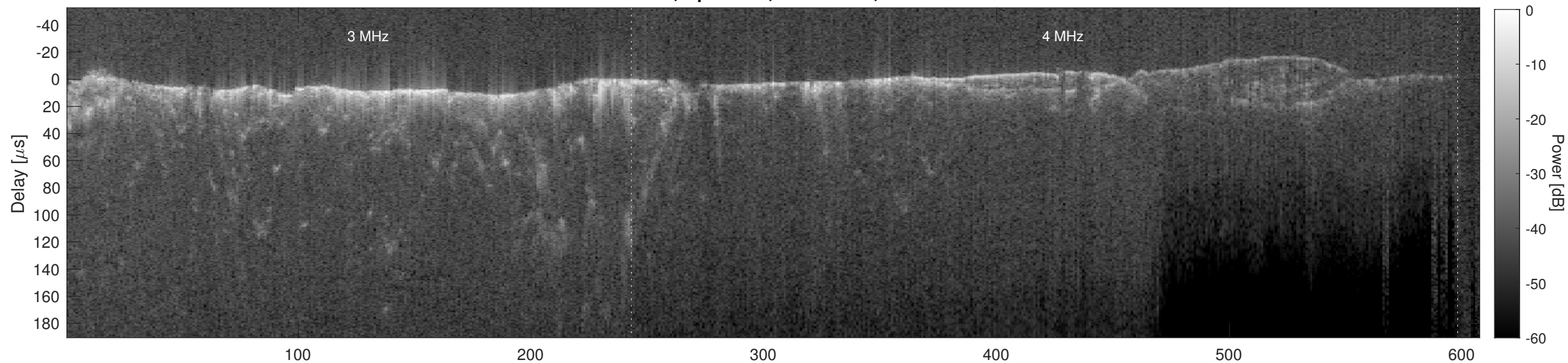
Orbit 21264, Cluttergram
