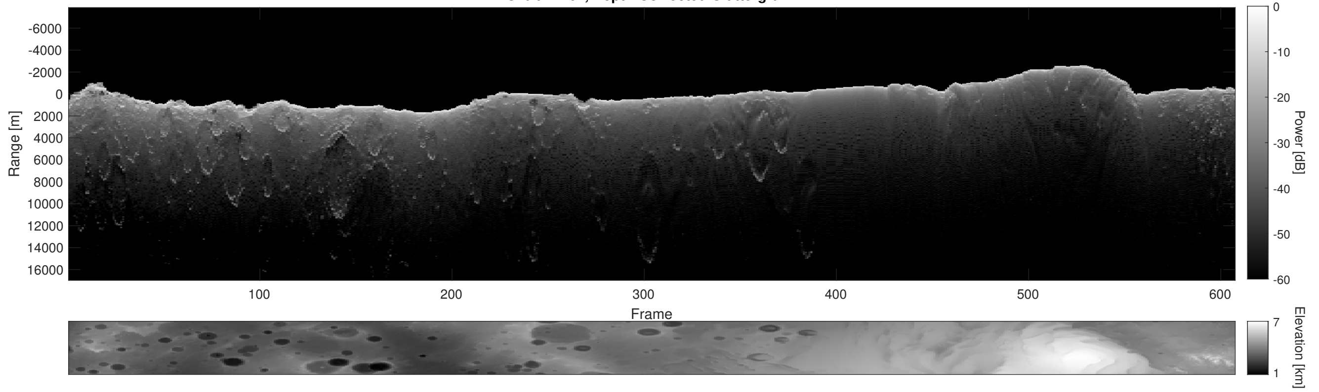
Orbit 21264, Depth-Corrected Cluttergram
