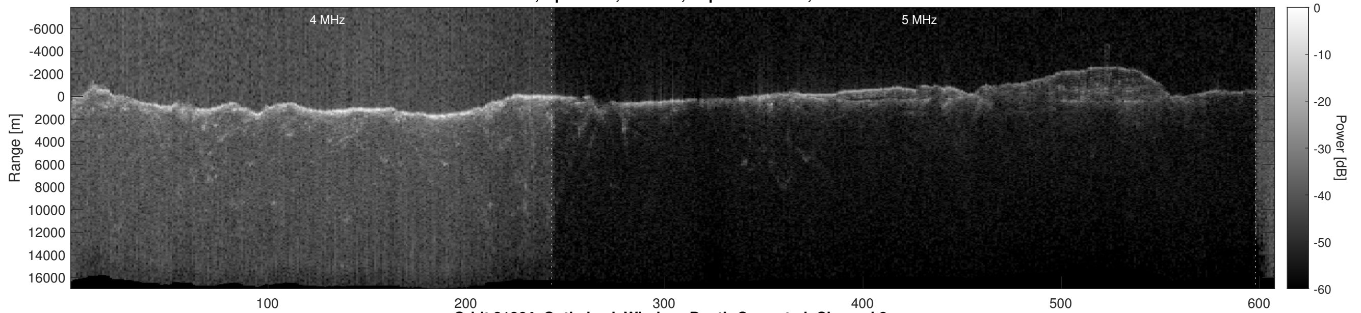
Orbit 21264, Optimized, Window, Depth-Corrected, Channel 2
