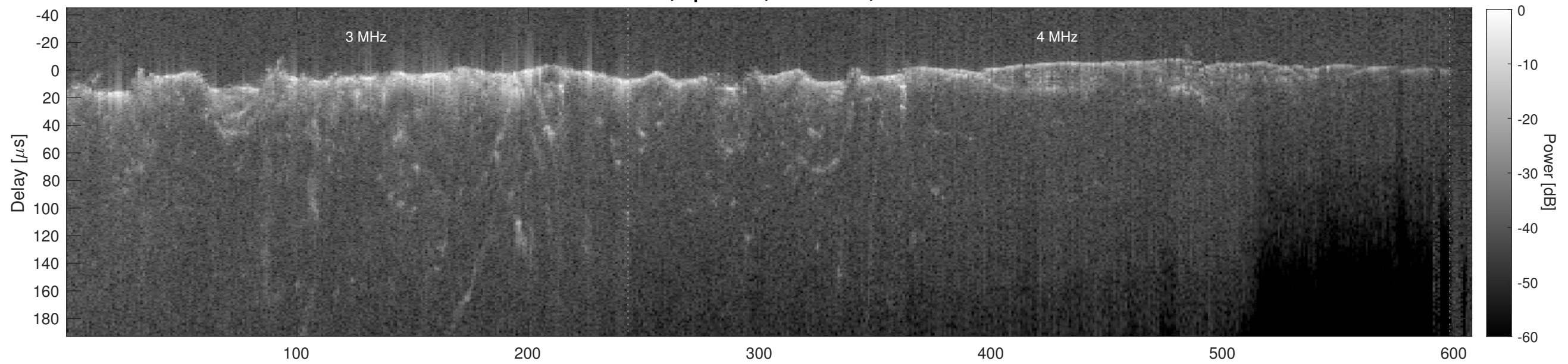
Orbit 21265, Cluttergram
