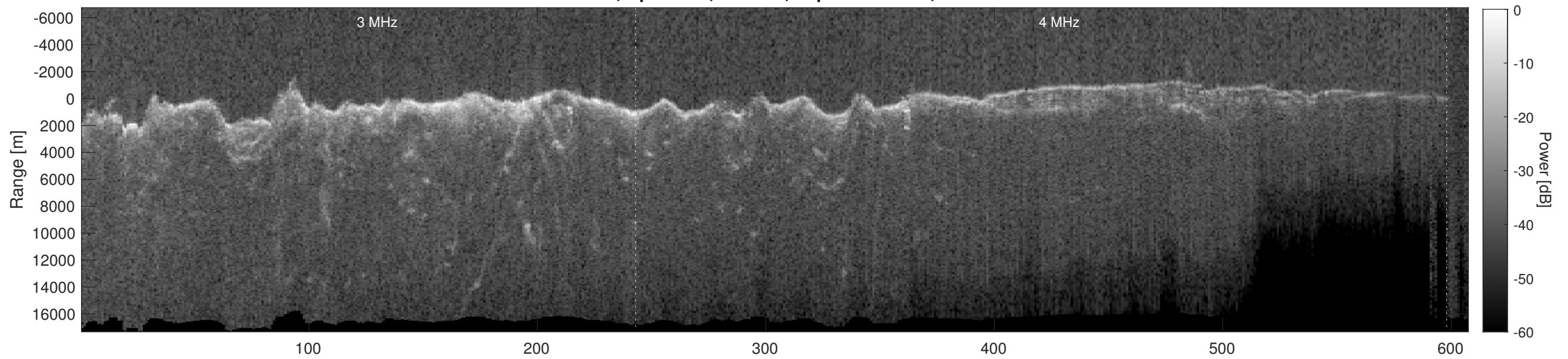
Orbit 21265, Depth-Corrected Cluttergram
