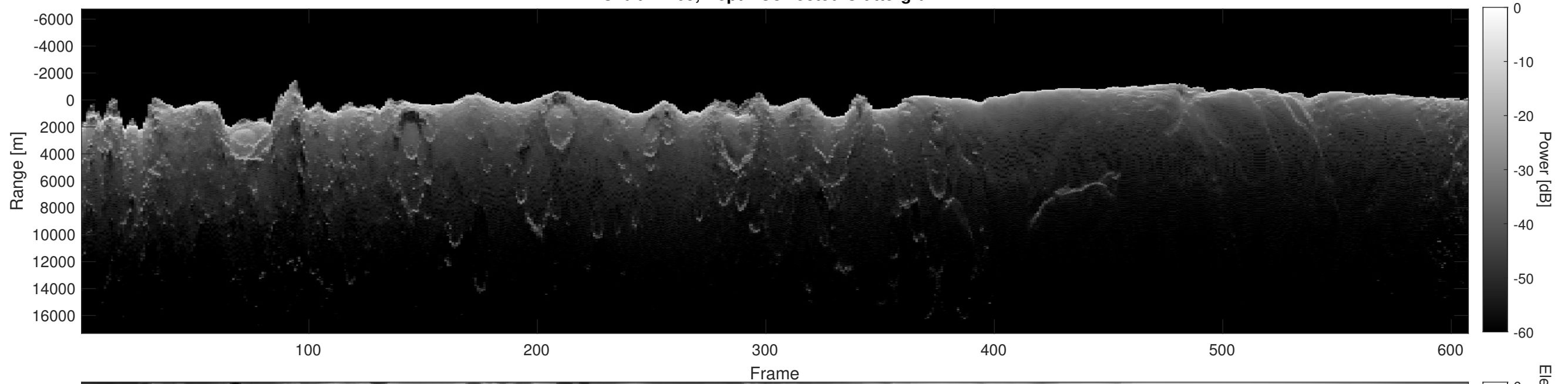
Orbit 21265, Depth-Corrected Cluttergram
