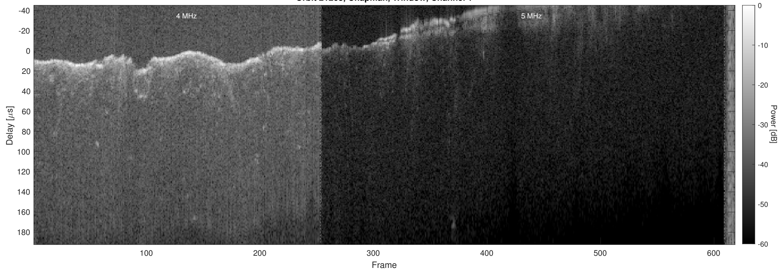
Orbit 21268, Chapman, Window, Channel 2
