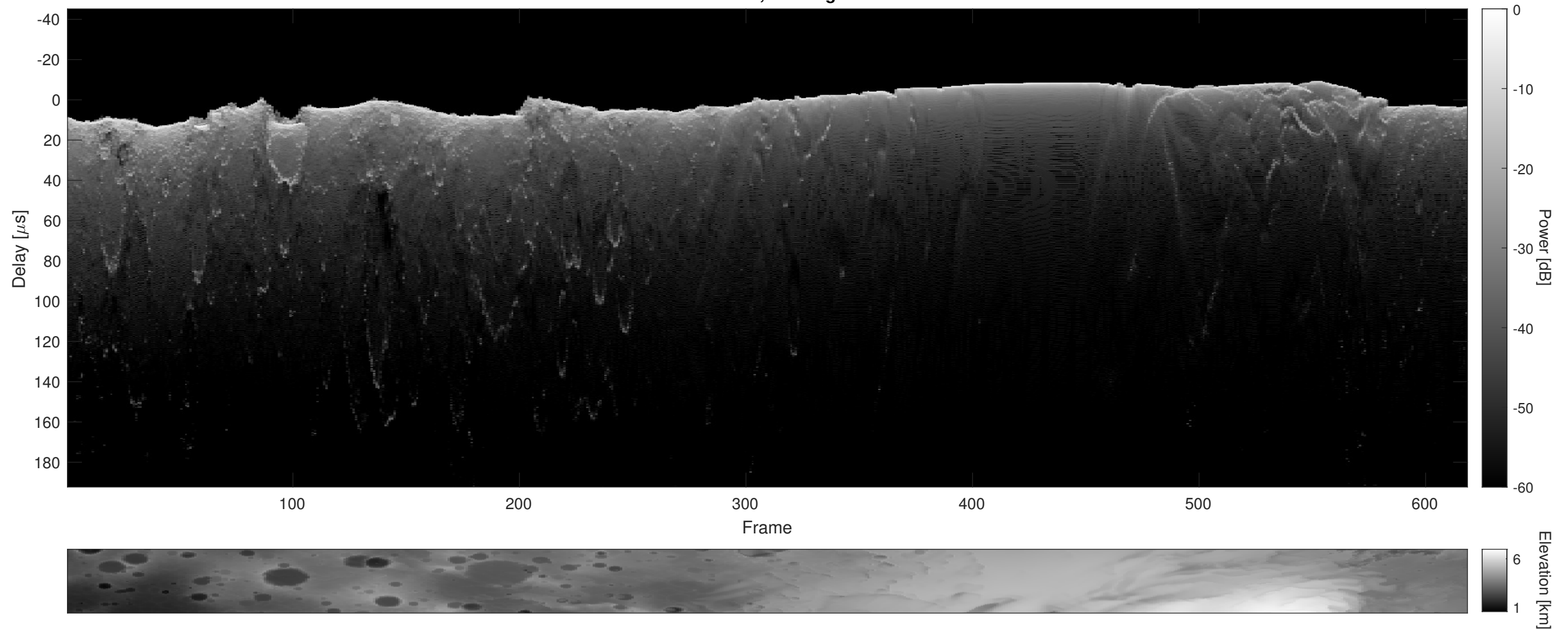
Orbit 21268, Cluttergram
