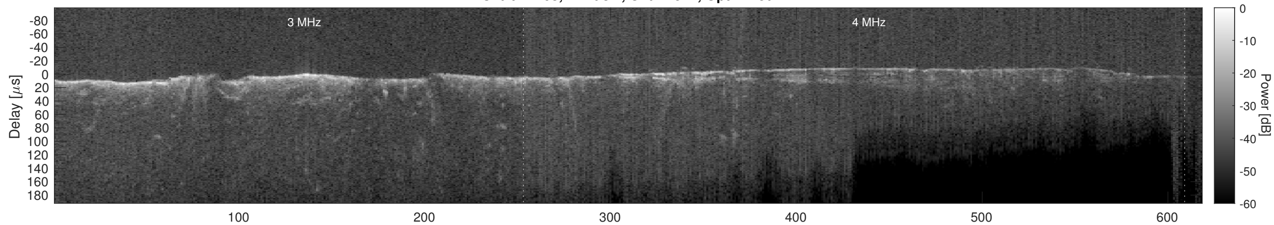
Orbit 21268, Cluttergram
