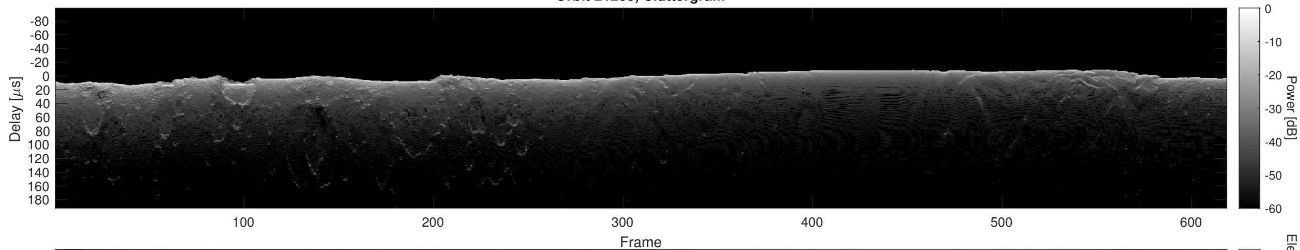
Orbit 21268, Cluttergram
