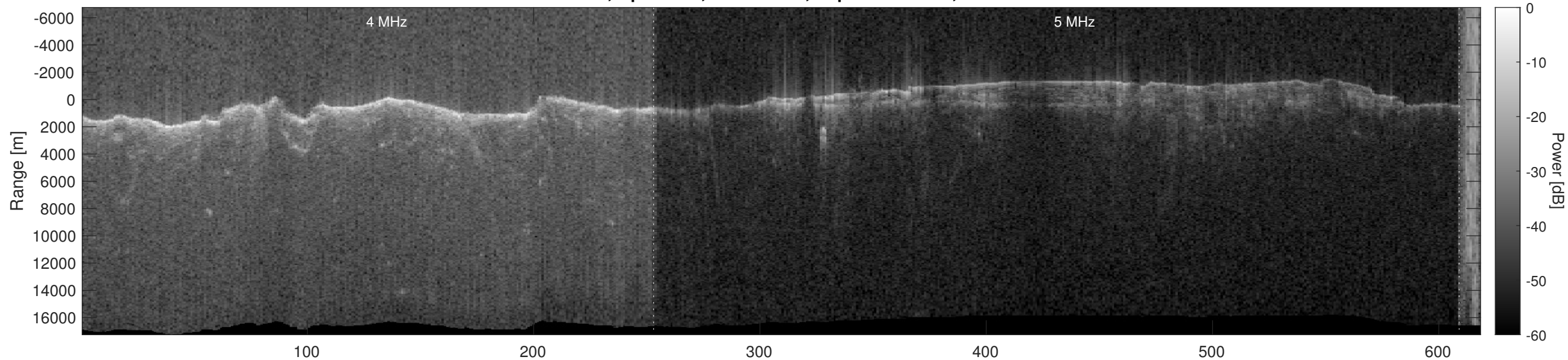
Orbit 21268, Optimized, No Window, Depth-Corrected, Channel 2
