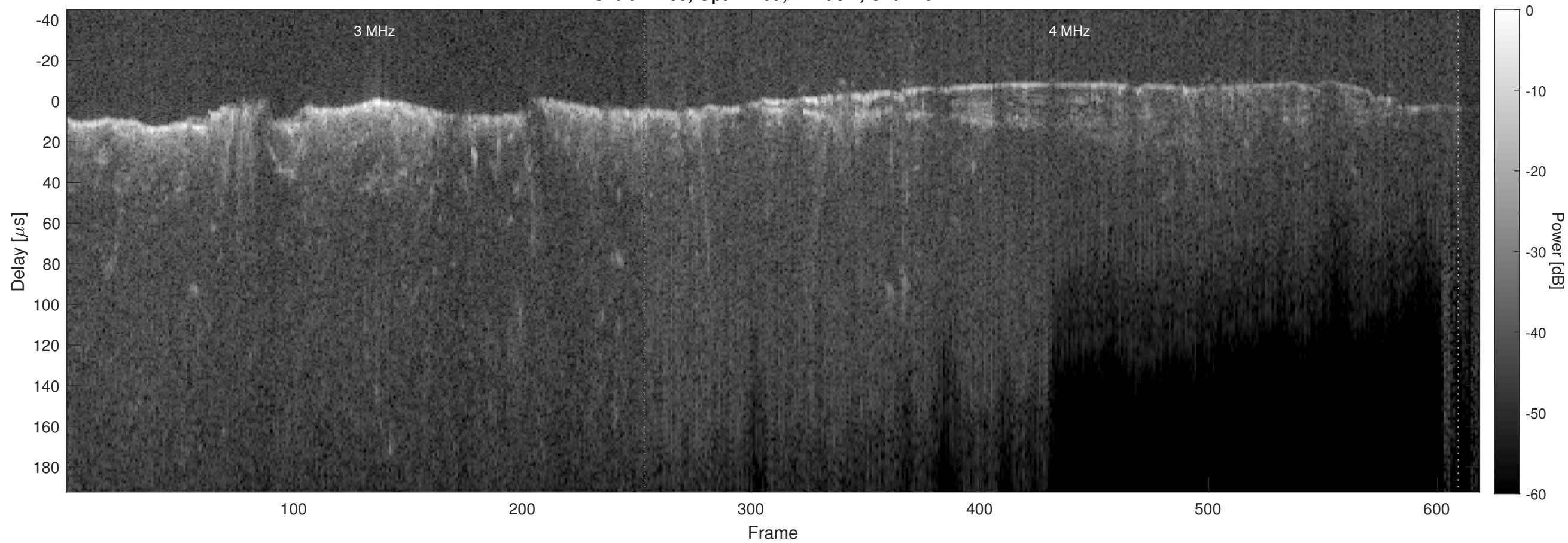
Orbit 21268, Optimized, Window, Channel 2
