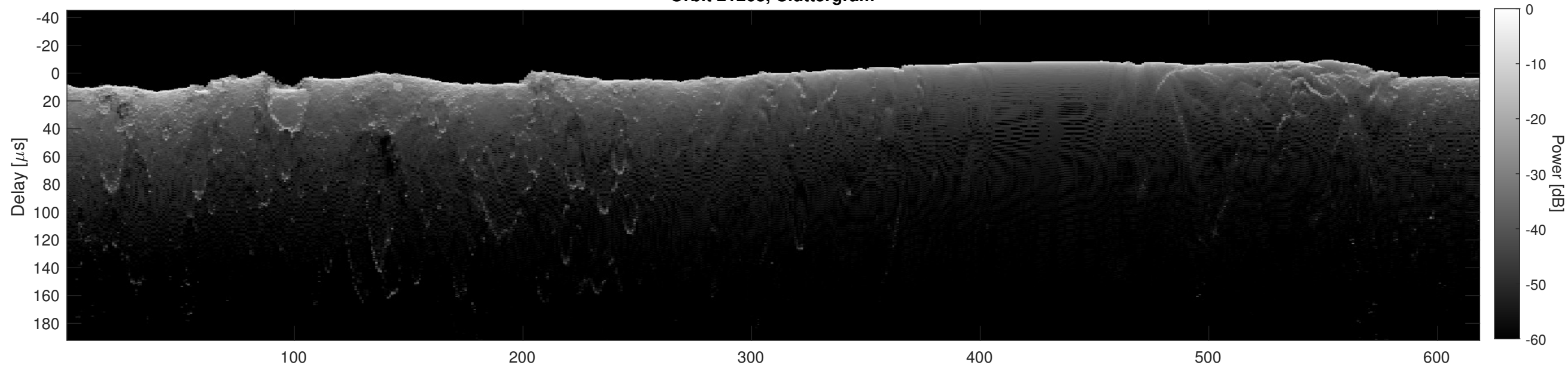
Orbit 21268, Cluttergram
