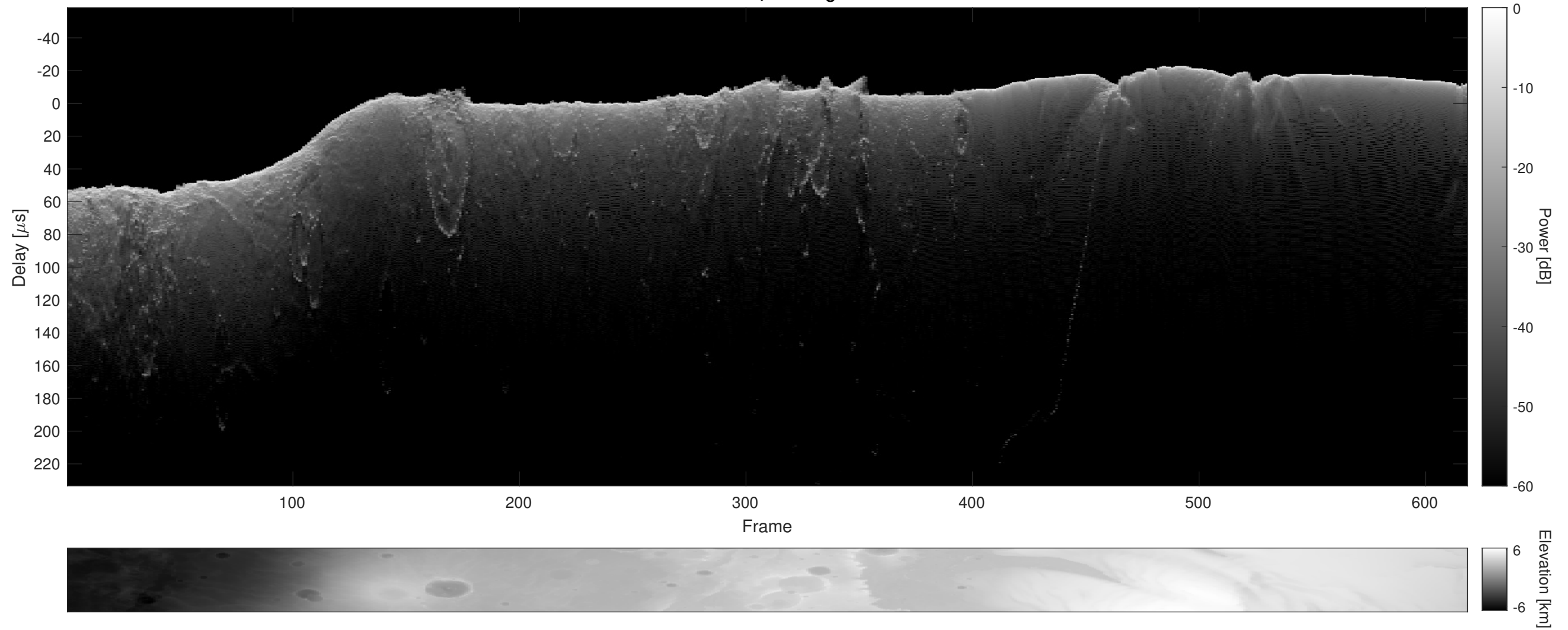
Orbit 21269, Cluttergram
