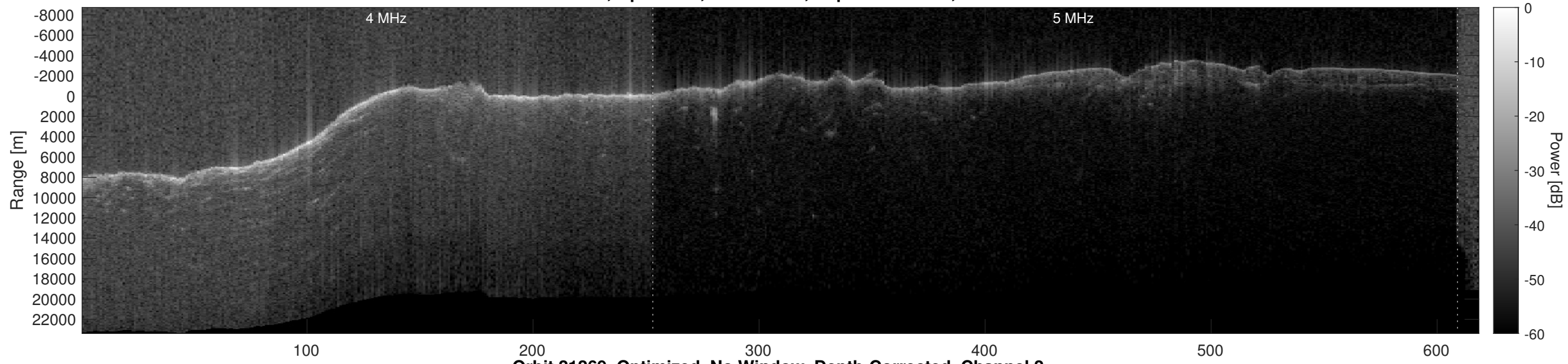
Orbit 21269, Optimized, No Window, Depth-Corrected, Channel 2
