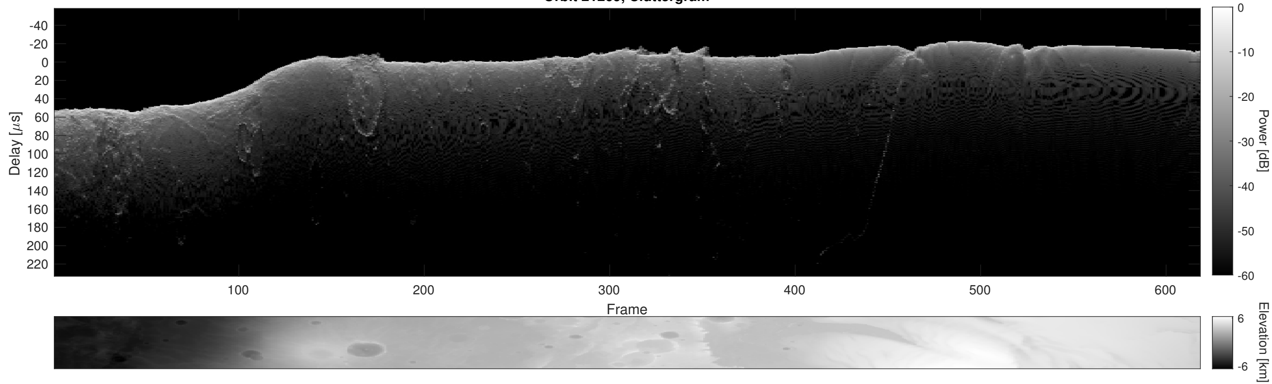
Orbit 21269, Cluttergram
