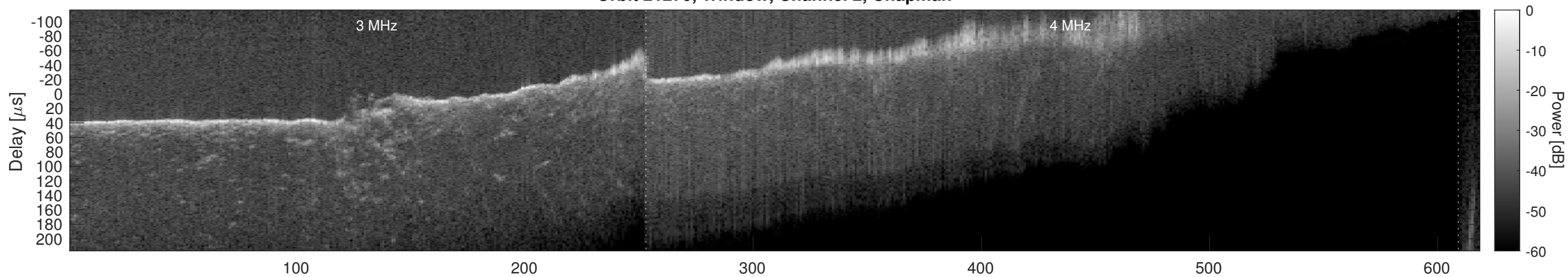
Orbit 21270, Window, Channel 2, Optimized
