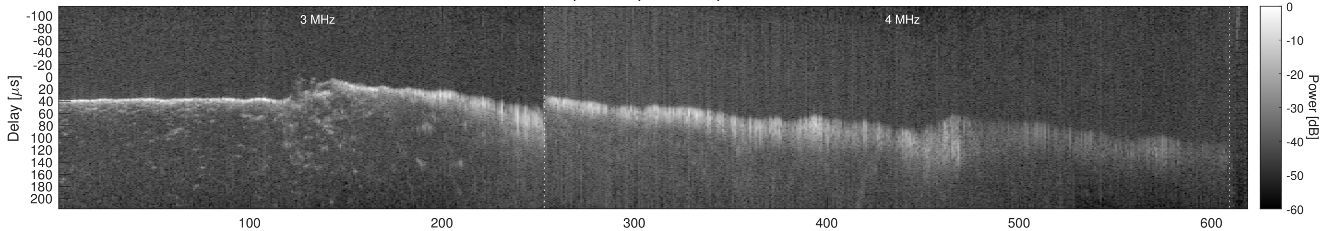
Orbit 21270, Window, Channel 2, Chapman
