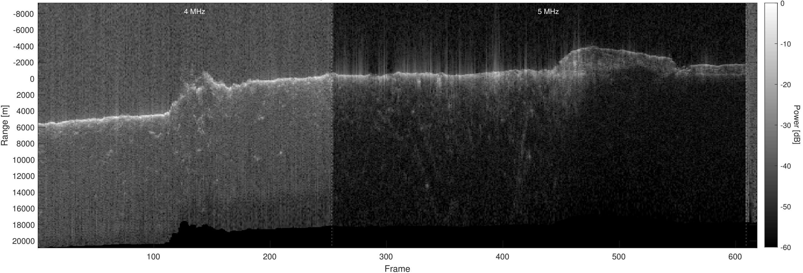
Orbit 21270, Optimized, No Window, Depth-Corrected, Channel 2
