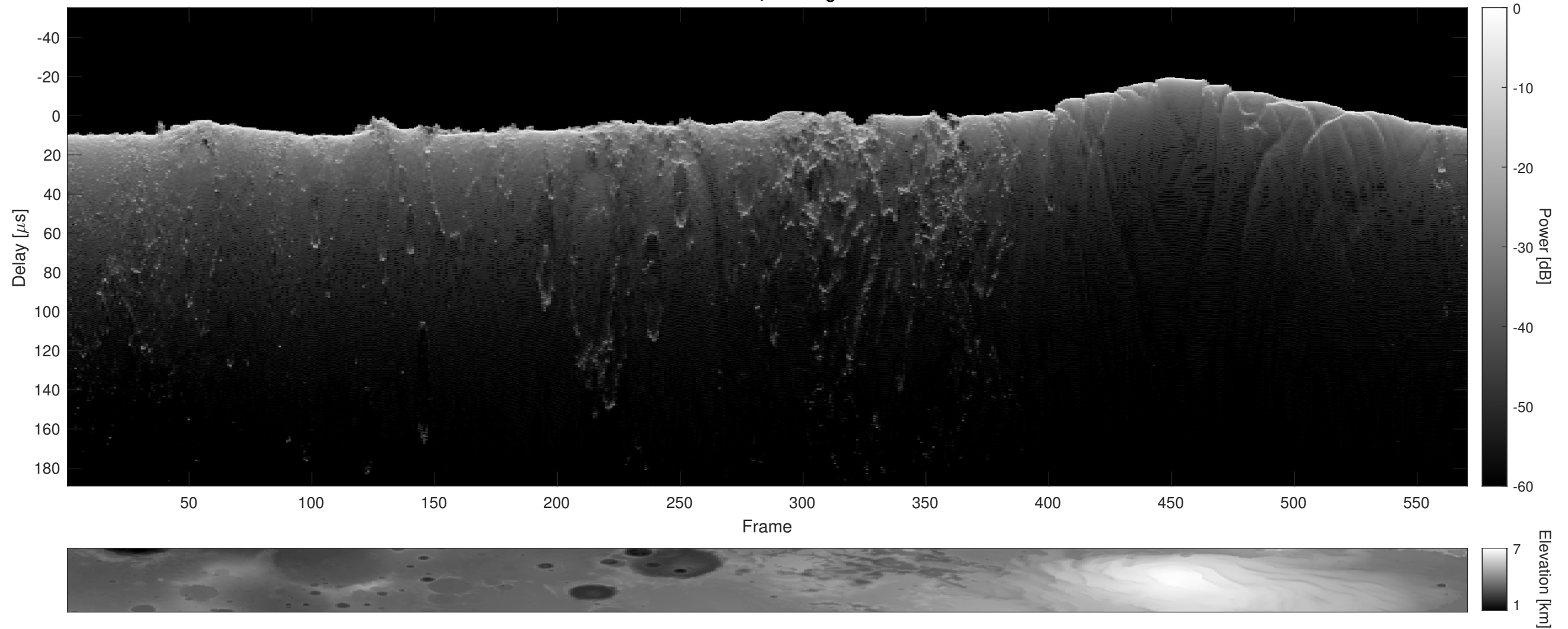
Orbit 21274, Cluttergram
