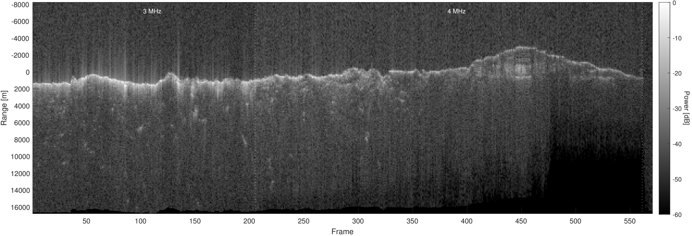
Orbit 21274, Optimized, No Window, Depth-Corrected, Channel 2
