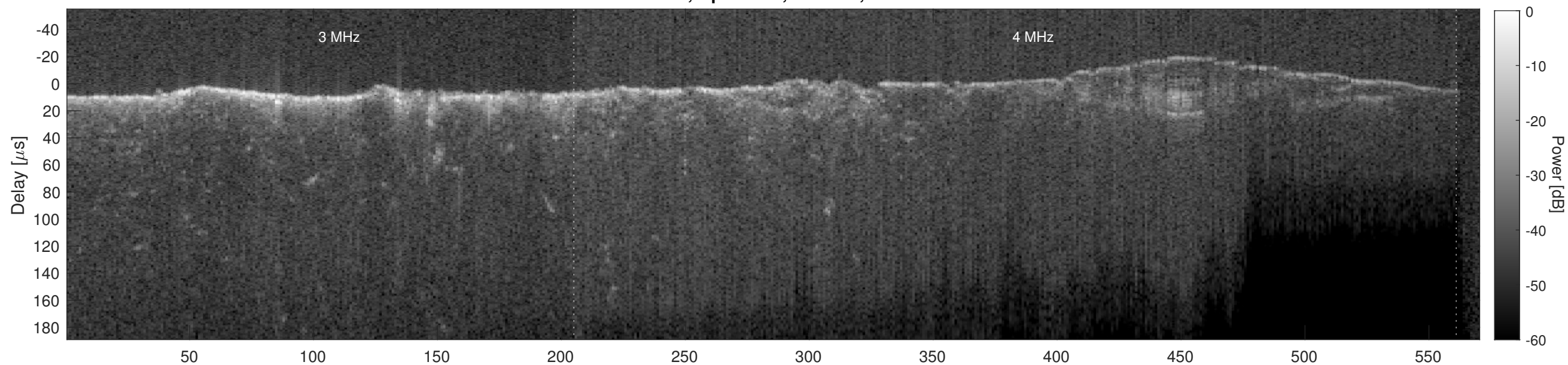
Orbit 21274, Cluttergram
