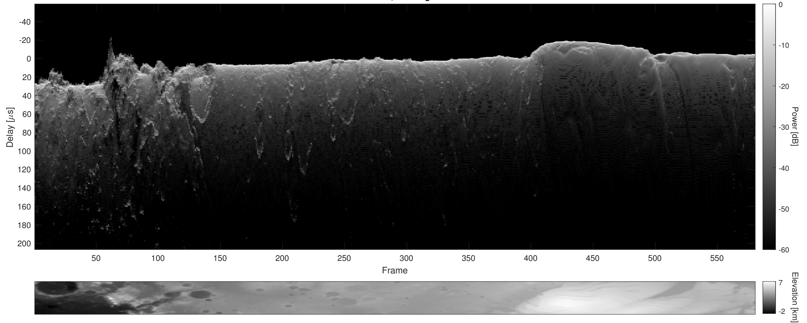
Orbit 21277, Cluttergram
