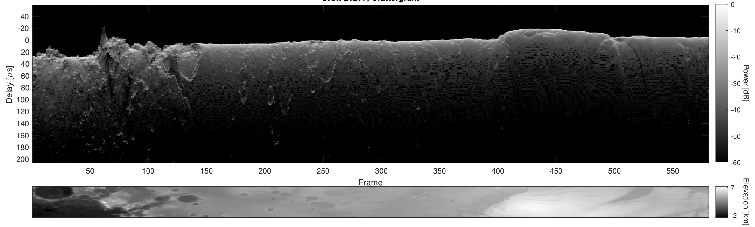
Orbit 21277, Cluttergram
