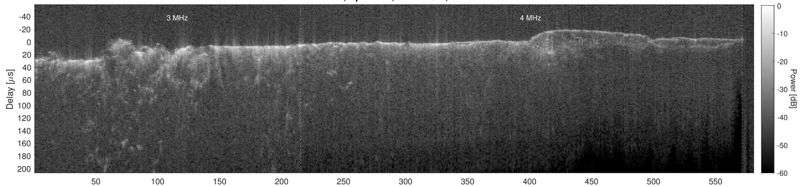
Orbit 21277, Cluttergram
