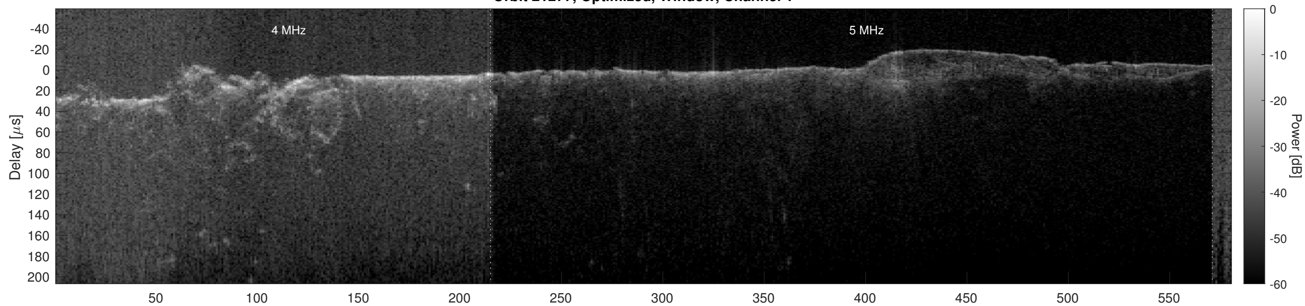
Orbit 21277, Optimized, Window, Channel 2
