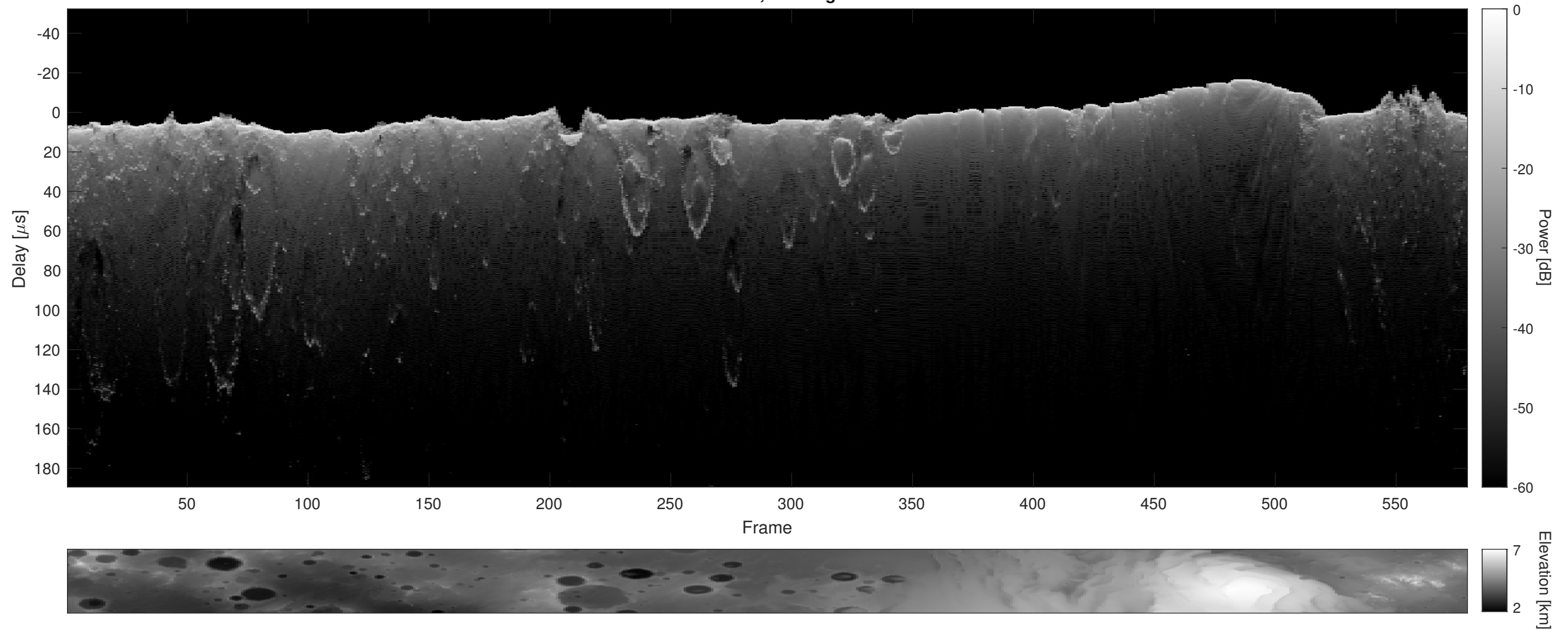
Orbit 21278, Cluttergram
