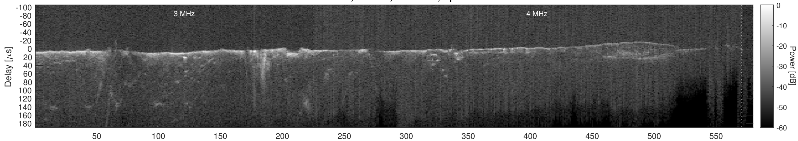
Orbit 21278, Cluttergram
