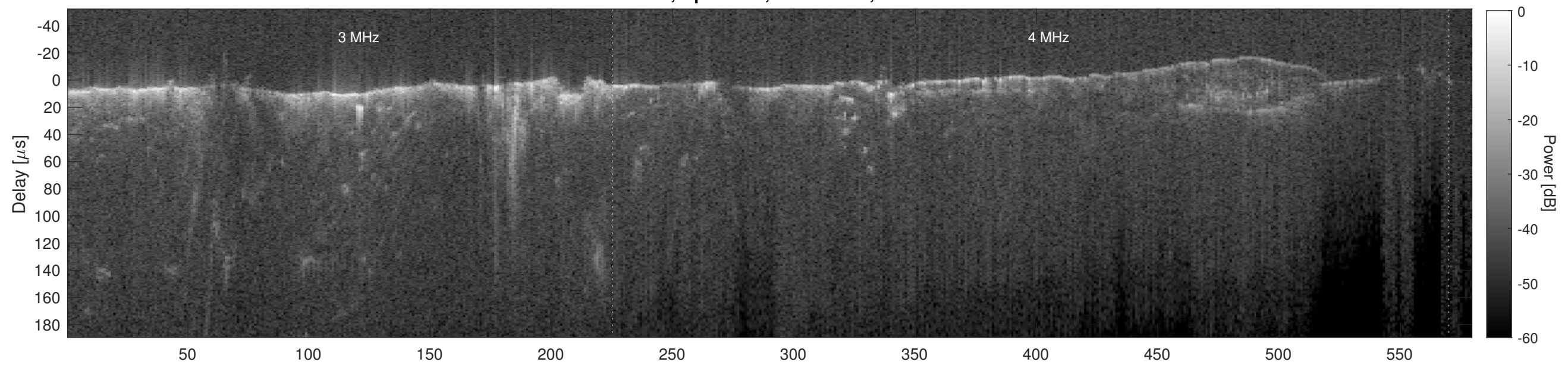
Orbit 21278, Cluttergram
