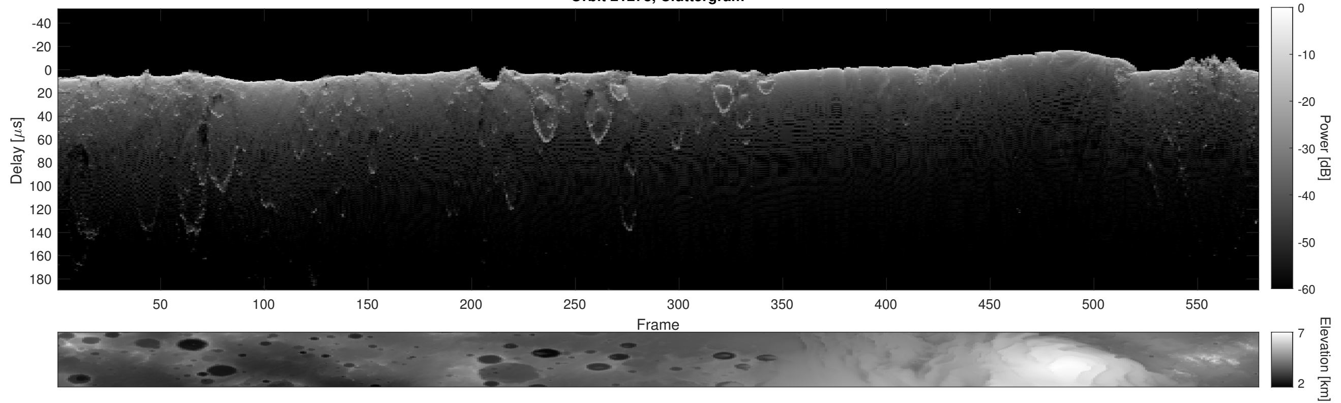
Orbit 21278, Cluttergram
