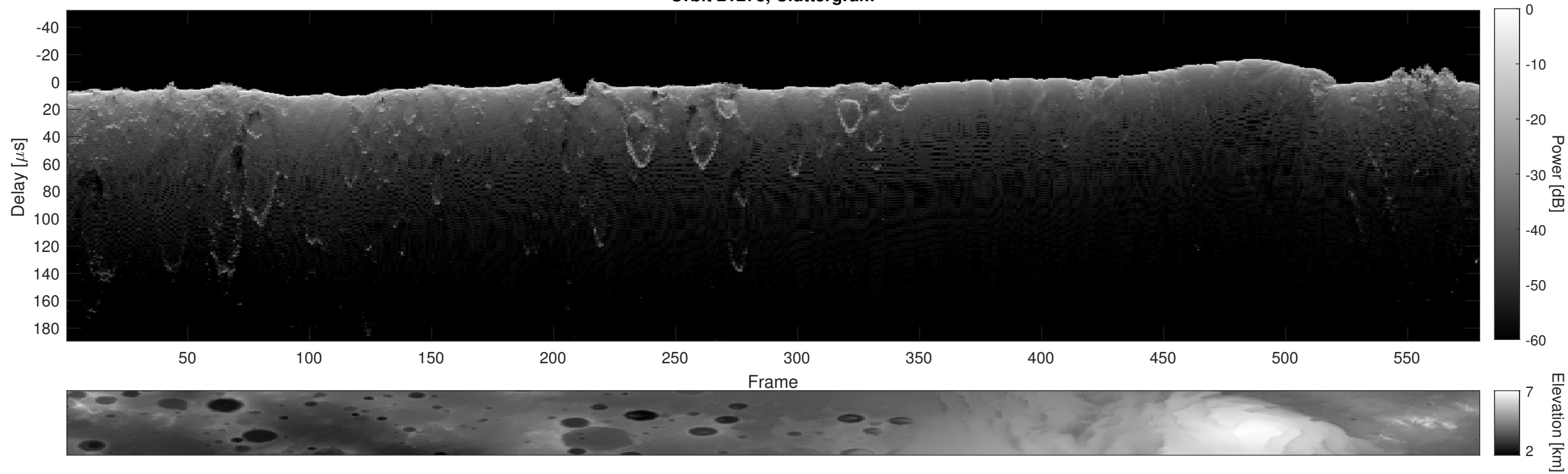
Orbit 21278, Cluttergram
