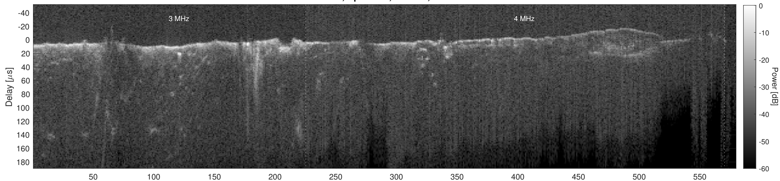
Orbit 21278, Cluttergram
