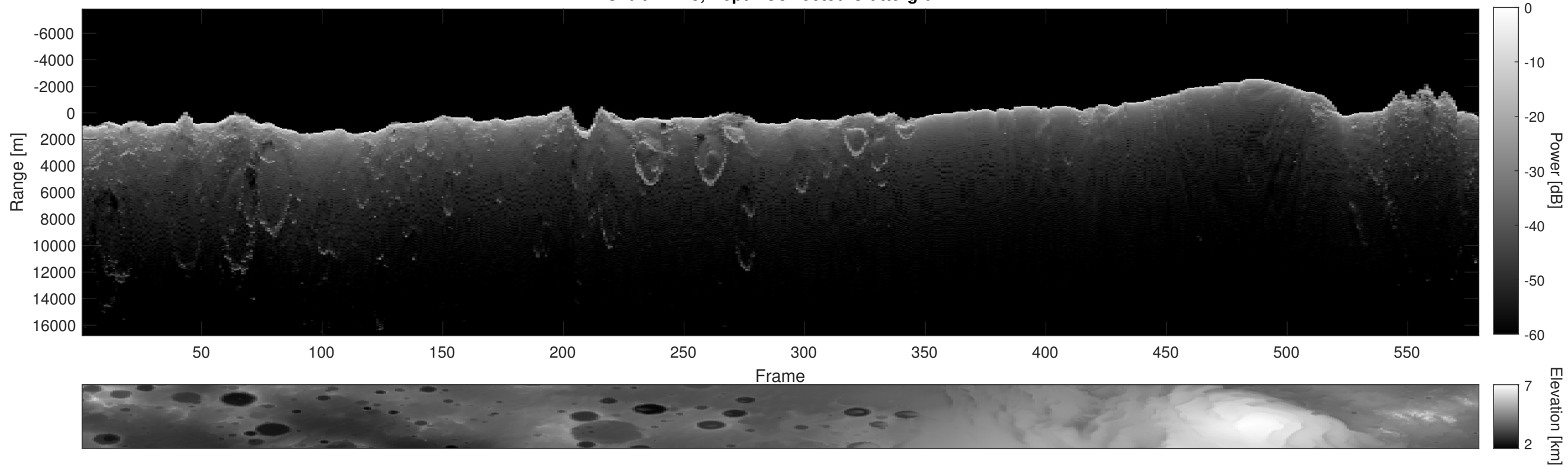
Orbit 21278, Depth-Corrected Cluttergram
