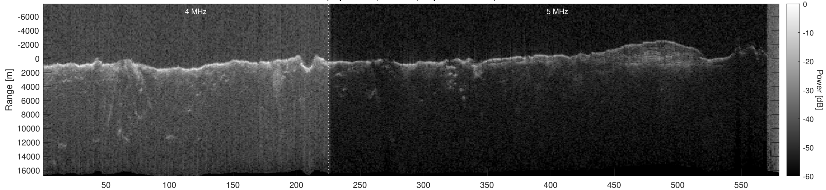
Orbit 21278, Optimized, Window, Depth-Corrected, Channel 2
