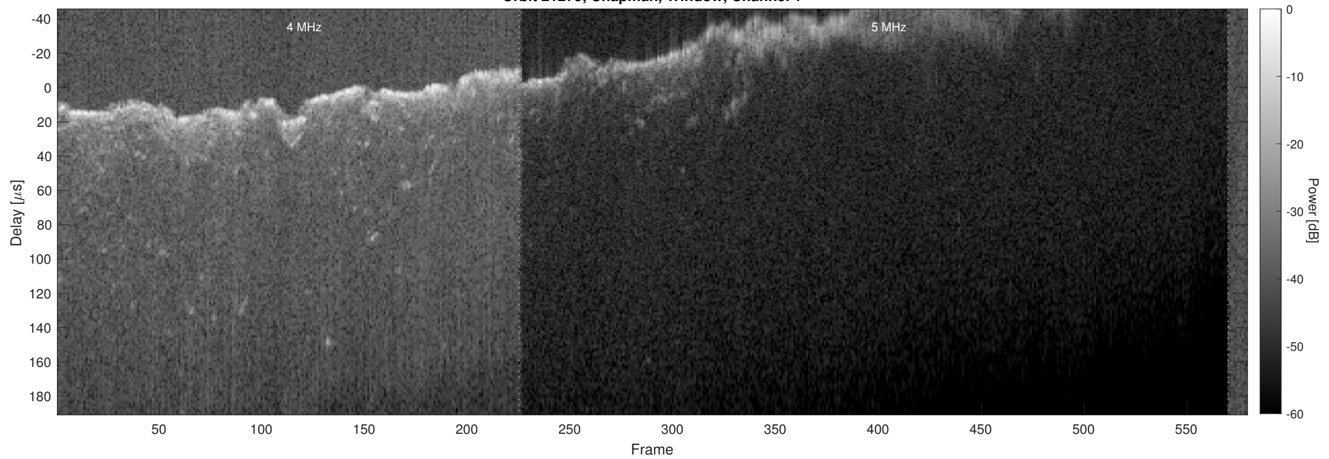
Orbit 21279, Chapman, Window, Channel 2
