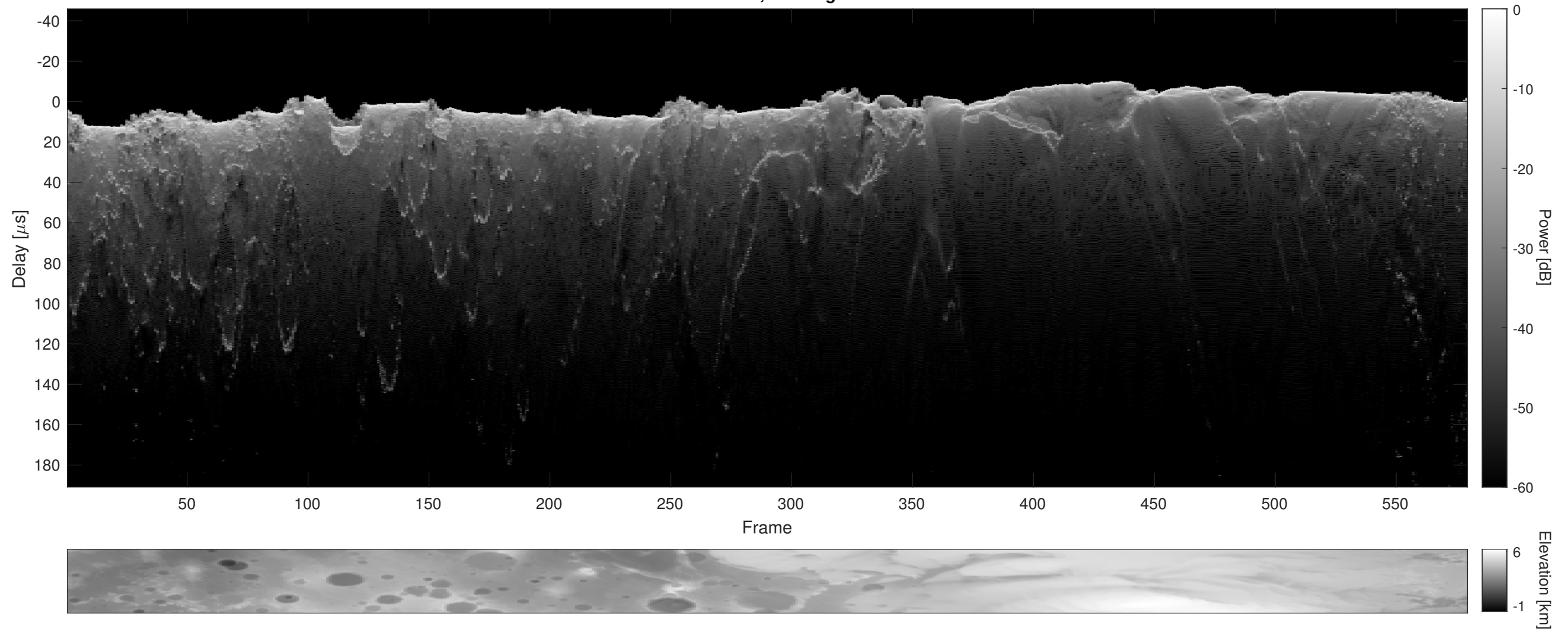
Orbit 21279, Cluttergram
