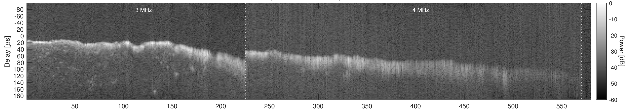
Orbit 21279, Window, Channel 2, Chapman
