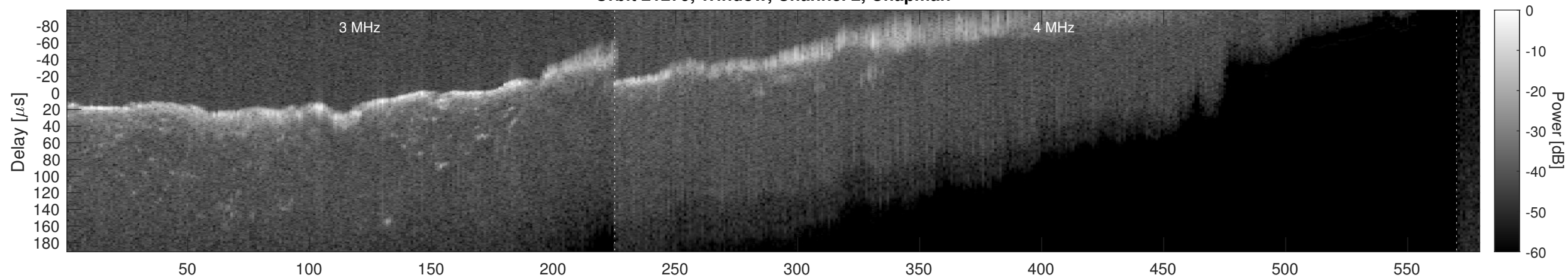
Orbit 21279, Window, Channel 2, Optimized
