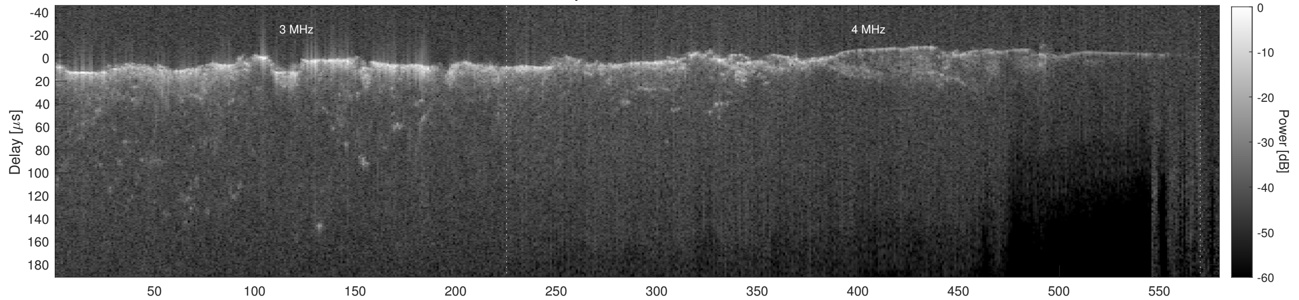
Orbit 21279, Cluttergram
