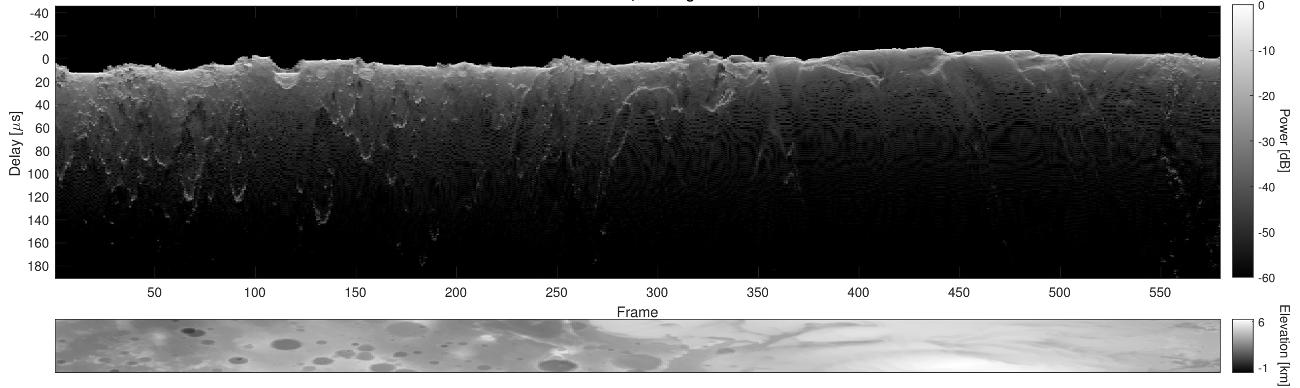
Orbit 21279, Cluttergram
