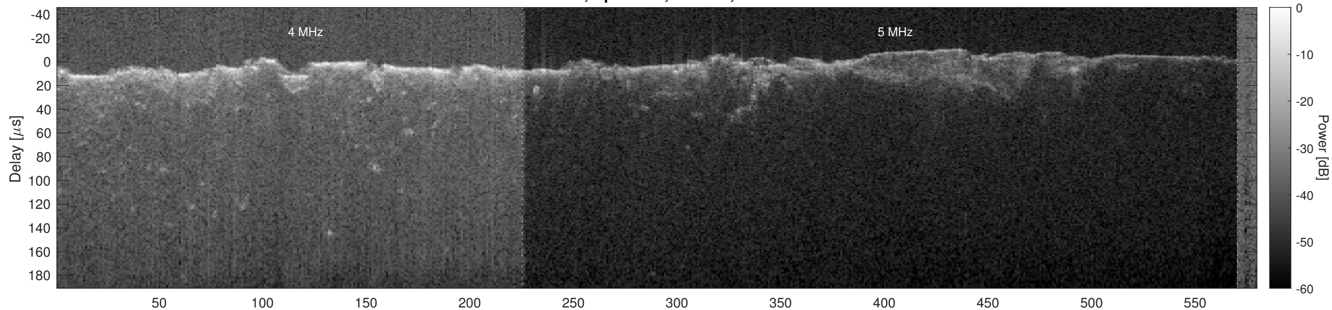
Orbit 21279, Optimized, Window, Channel 2
