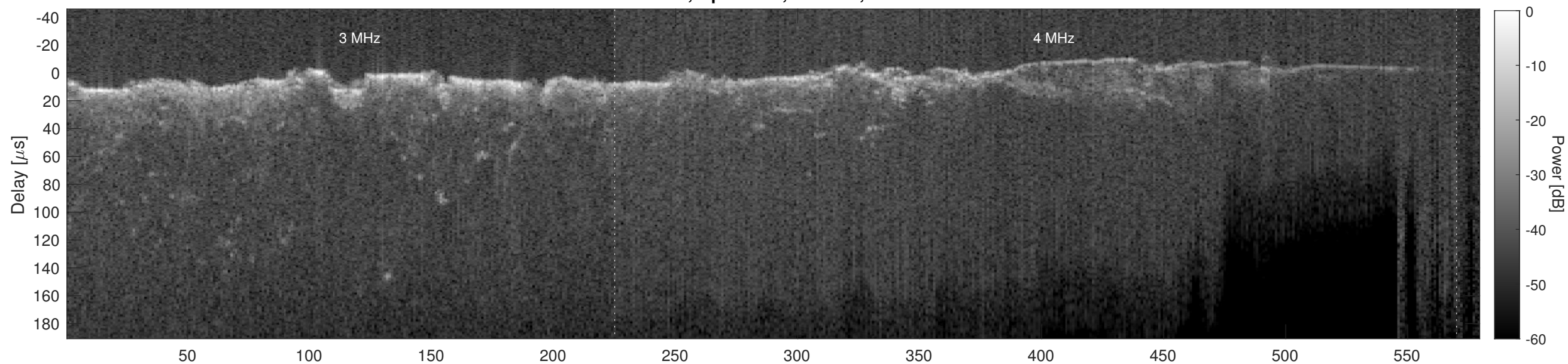
Orbit 21279, Cluttergram
