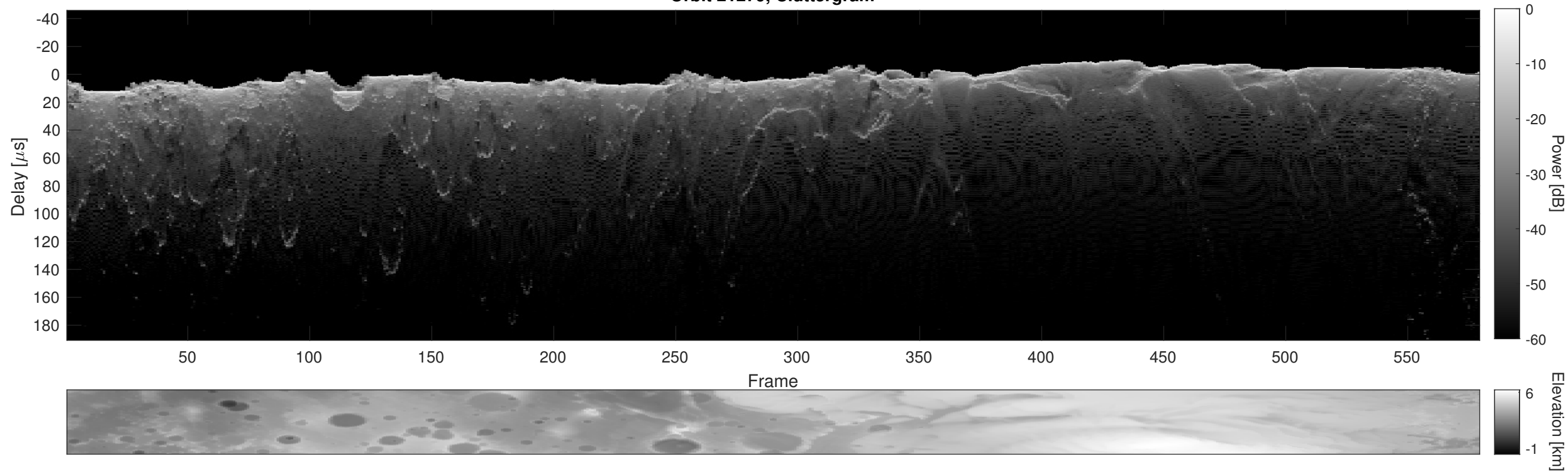
Orbit 21279, Cluttergram
