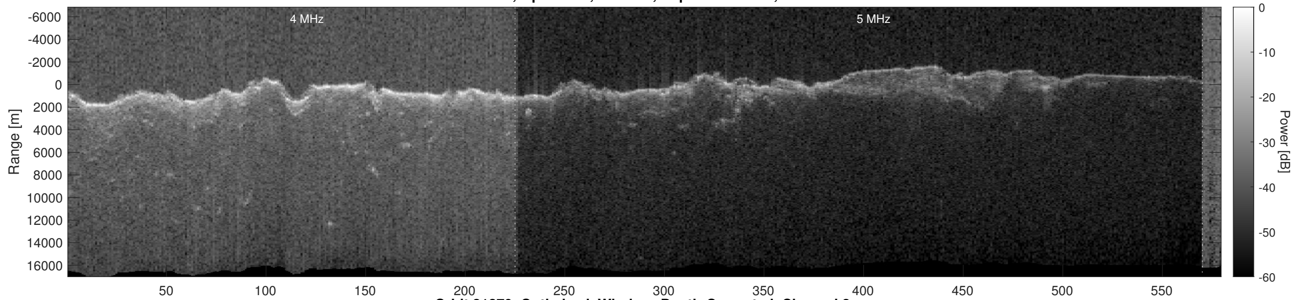
Orbit 21279, Optimized, Window, Depth-Corrected, Channel 2
