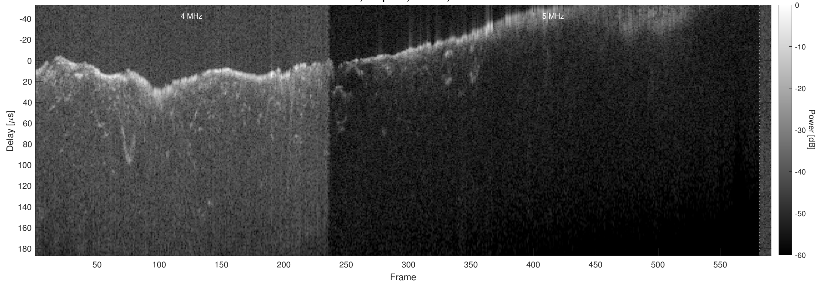
Orbit 21285, Chapman, Window, Channel 2
