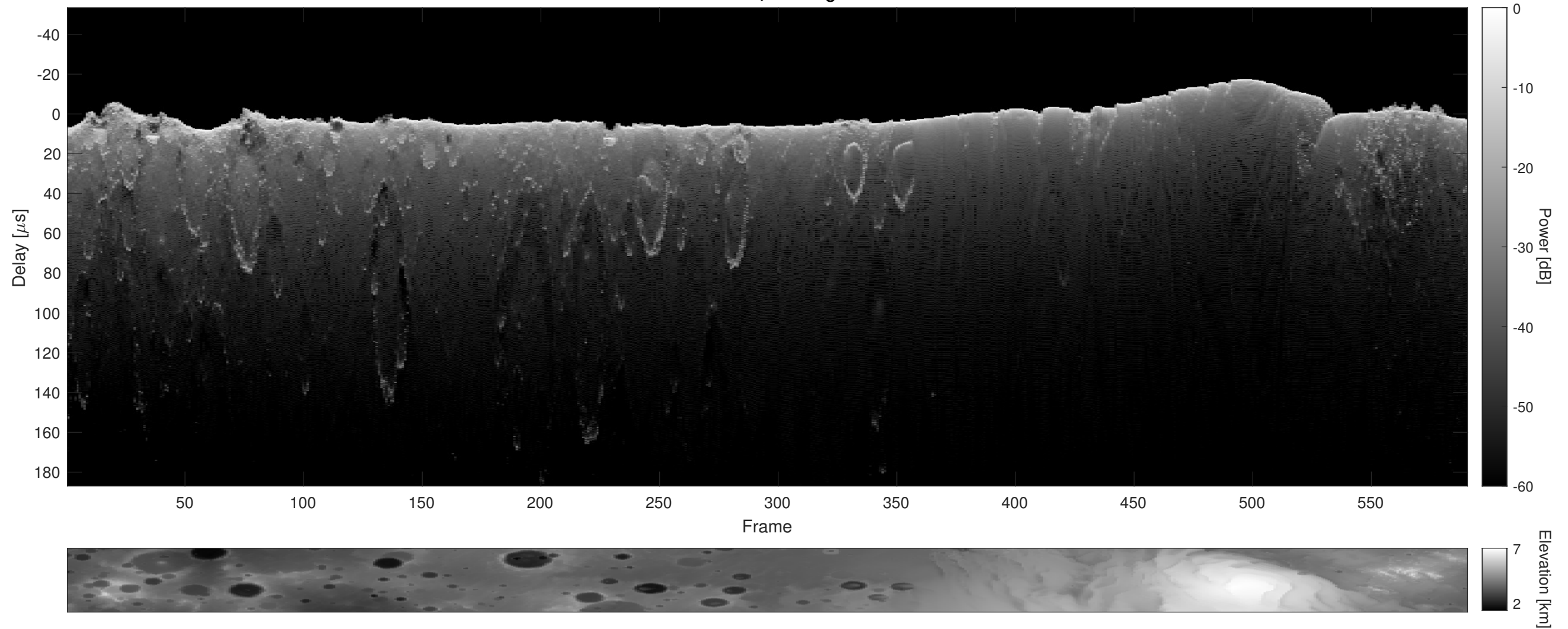
Orbit 21285, Cluttergram
