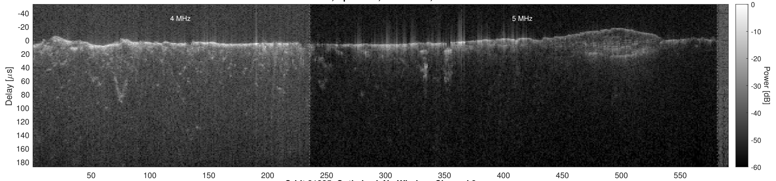
Orbit 21285, Optimized, No Window, Channel 2
