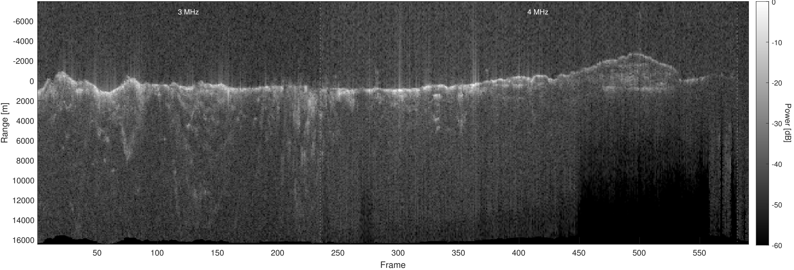
Orbit 21285, Optimized, No Window, Depth-Corrected, Channel 2
