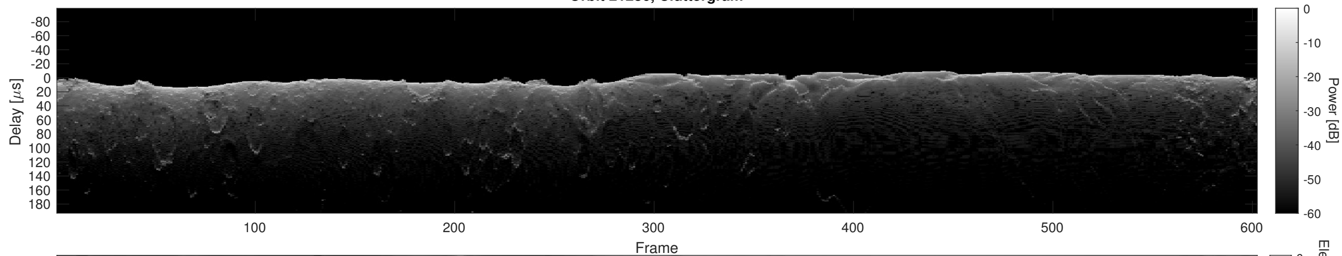
Orbit 21286, Cluttergram
