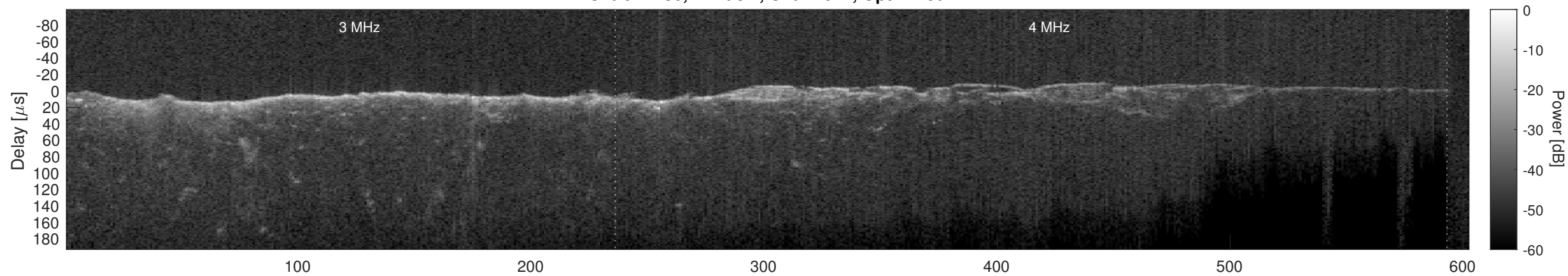
Orbit 21286, Cluttergram
