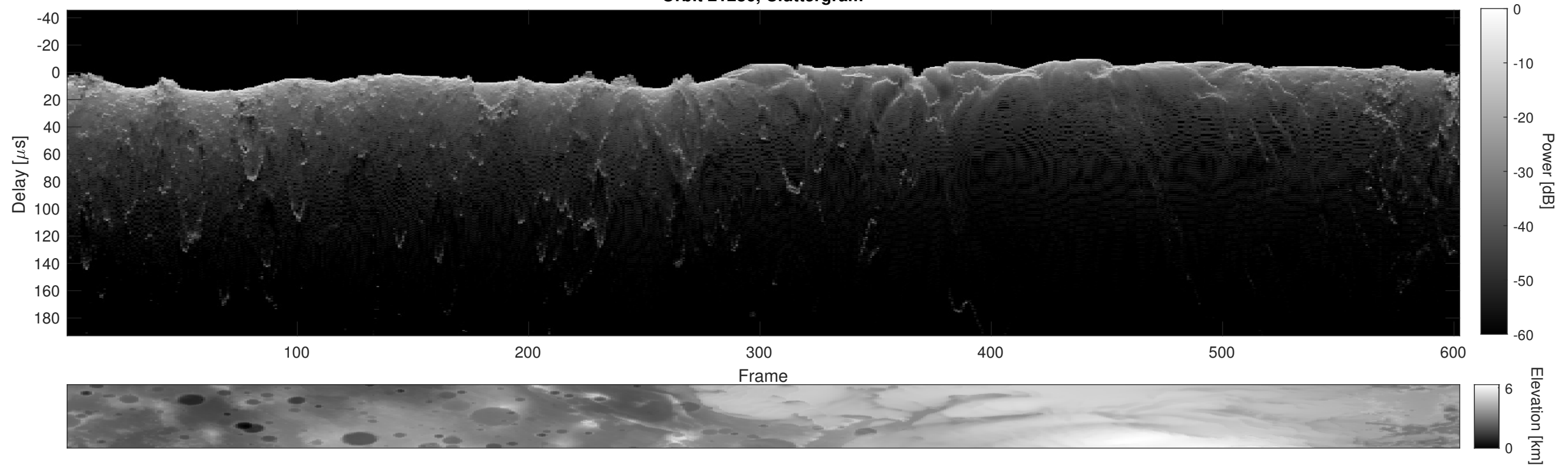
Orbit 21286, Cluttergram
