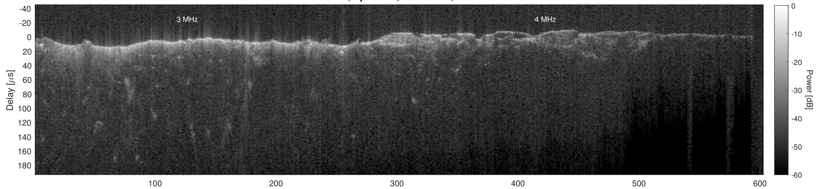
Orbit 21286, Cluttergram
