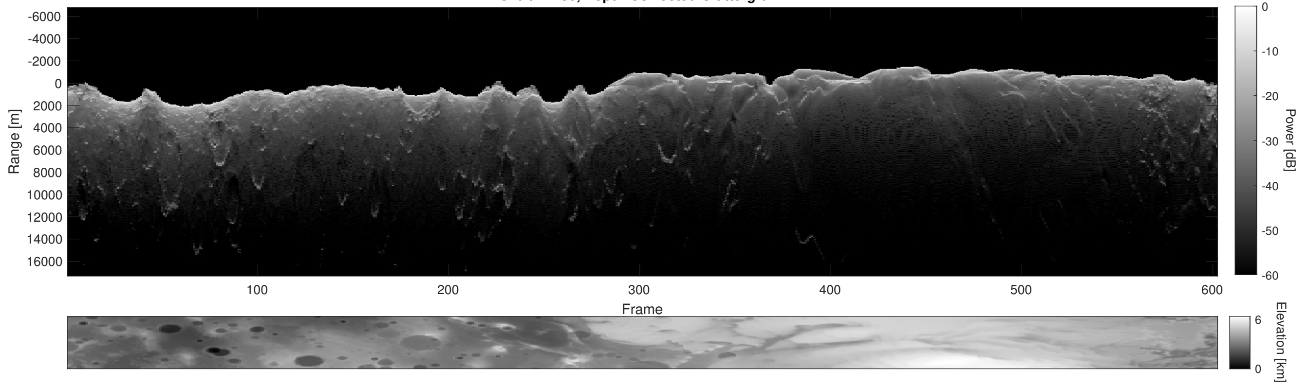
Orbit 21286, Depth-Corrected Cluttergram
