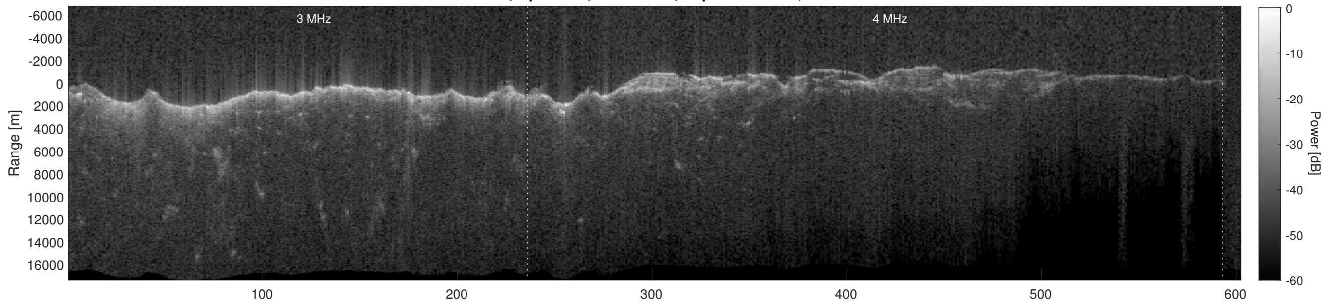
Orbit 21286, Depth-Corrected Cluttergram
